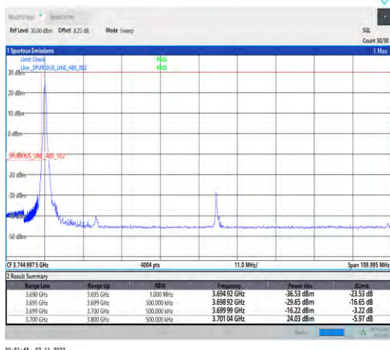
1-N78-3700-3800-PC2-30-100-L-1-DFT-PI2BPSK-Edge_1RB_Left-1@0-Ant1-1--PASS-see graph
