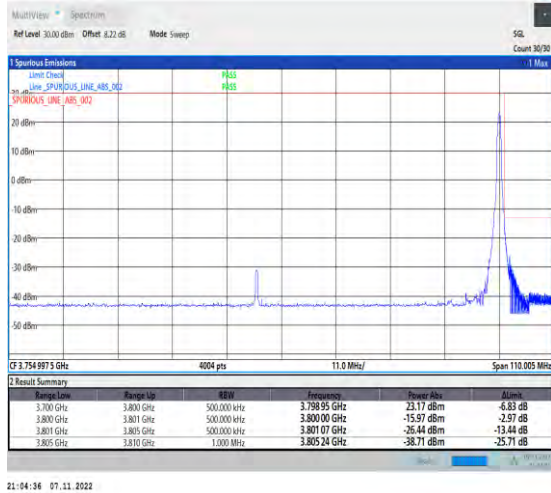
1-N78-3700-3800-PC2-30-100-H-2-DFT-PI2BPSK-Edge_1RB_Right-1@272-Ant1-1--PASS-see graph
