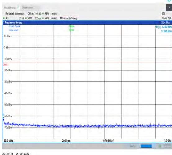
1-N78-3700-3800-PC2-30-100-L-1-DFT-PI2BPSK-In ner_1RB_Left-1@1-30-1000-Ant1-31.94--62.26--13- PASS
