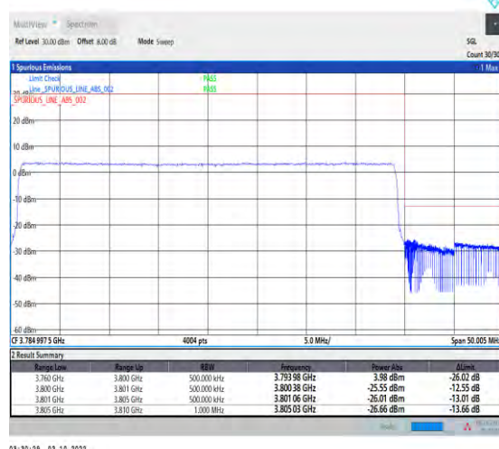
1-N78-3700-3800-PC2-30-40-H-6-CP-QPSK-Outer_Full-106@0-Ant1-1--PASS-see graph
