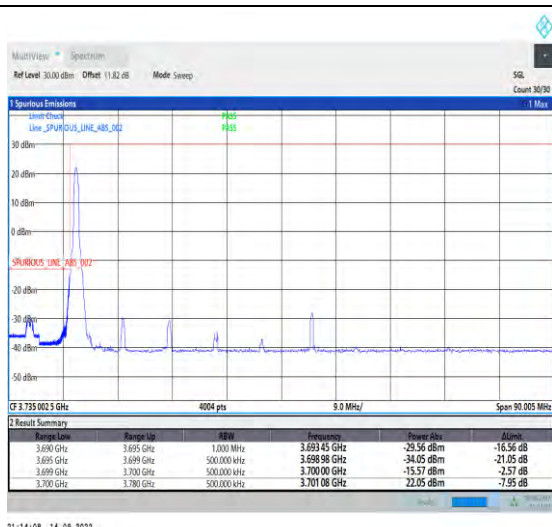
1-N78-3700-3800-PC2-30-80-L-1-DFT-PI2BPSK-Edge_1RB_Left-1@0-Ant1-1--PASS-see graph
