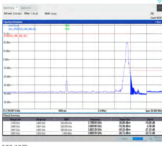
1-N78-3700-3800-PC2-30-40-H-5-CP-QPSK-Edge_1RB_Right-1@105-Ant1-1--PASS-see graph
