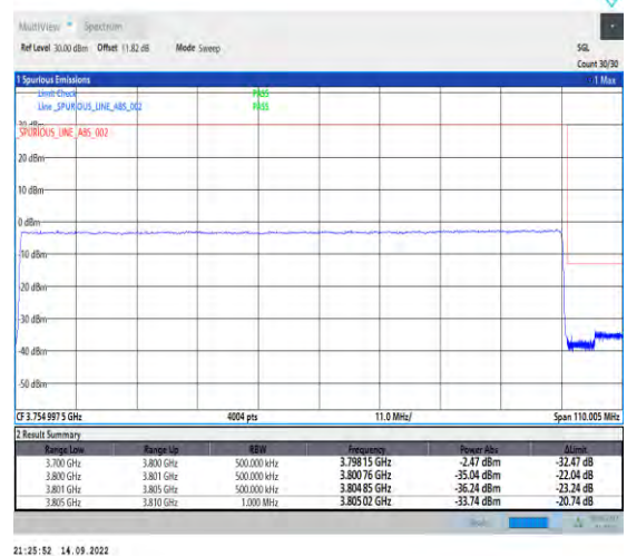
1-N78-3700-3800-PC2-30-100-H-6-CP-QPSK-Outer_Full-273@0-Ant1-1--PASS-see graph
