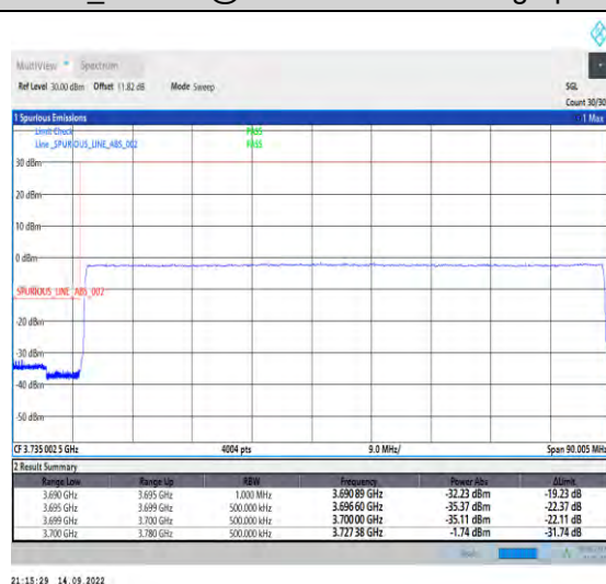
1-N78-3700-3800-PC2-30-80-L-6-CP-QPSK-Outer_Full-217@0-Ant1-1--PASS-see graph
