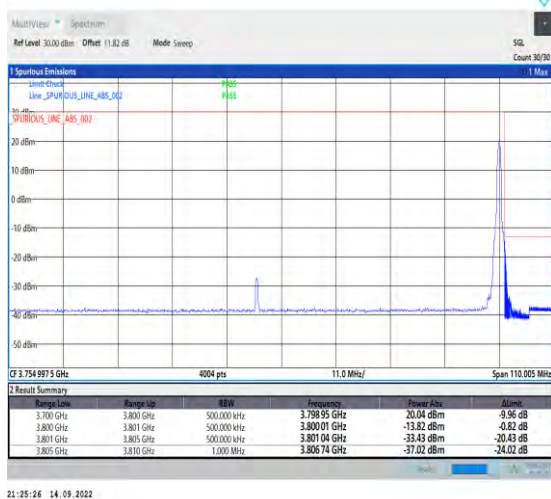
1-N78-3700-3800-PC2-30-100-H-5-CP-QPSK-Edge_1RB_Right-1@272-Ant1-1--PASS-see graph
