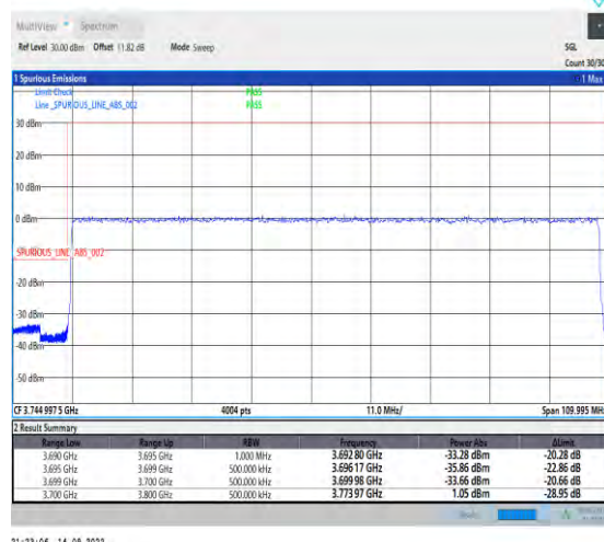
1-N78-3700-3800-PC2-30-100-L-3-DFT-PI2BPSK-Outer_Full-270@0-Ant1-1--PASS-see graph
