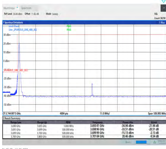
1-N78-3700-3800-PC2-30-100-L-4-CP-QPSK-Edge_1RB_Left-1@0-Ant1-1--PASS-see graph
