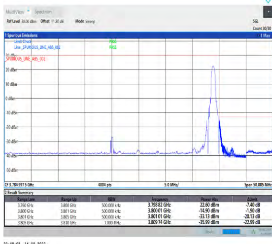
1-N78-3700-3800-PC2-30-40-H-2-DFT-PI2BPSK-Edge_1RB_Right-1@105-Ant1-1--PASS-see graph
