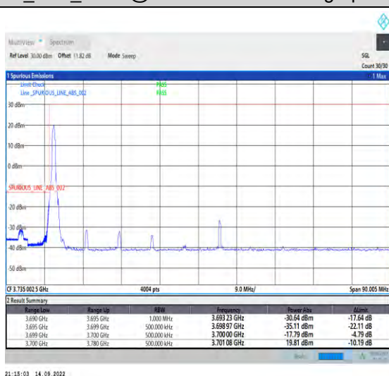
1-N78-3700-3800-PC2-30-80-L-4-CP-QPSK-Edge_1RB_Left-1@0-Ant1-1--PASS-see graph
