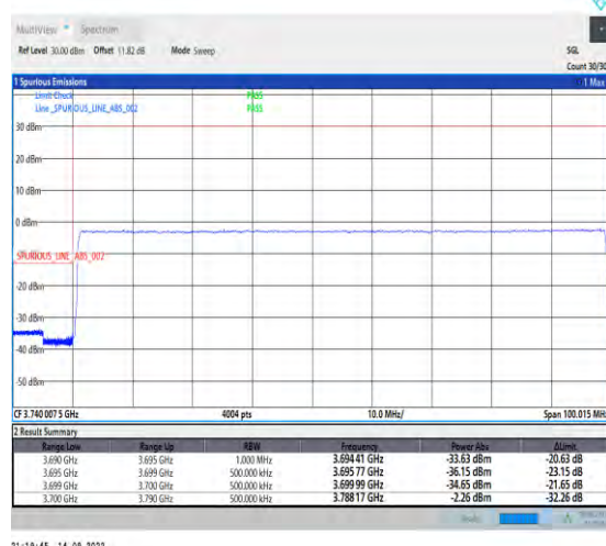
1-N78-3700-3800-PC2-30-90-L-6-CP-QPSK-Outer_Full-245@0-Ant1-1--PASS-see graph
