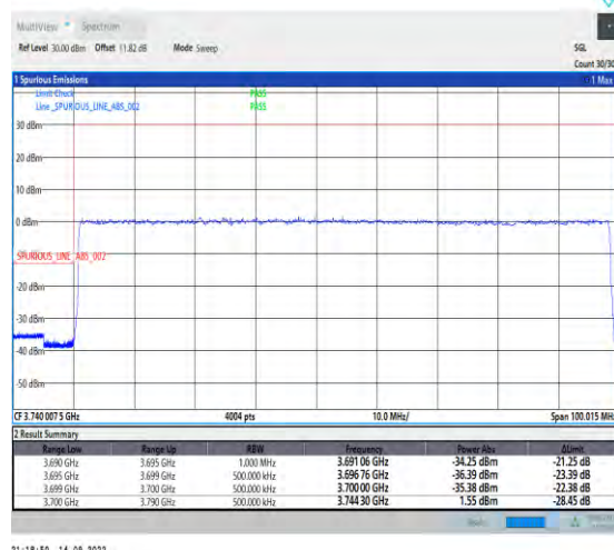
1-N78-3700-3800-PC2-30-90-L-3-DFT-PI2BPSK-Outer_Full-243@0-Ant1-1--PASS-see graph
