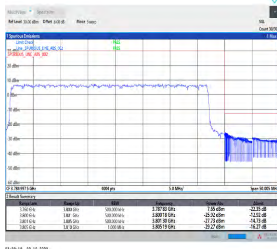
1-N78-3700-3800-PC2-30-40-H-3-DFT-PI2BPSK-Outer_Full-100@0-Ant1-1--PASS-see graph
