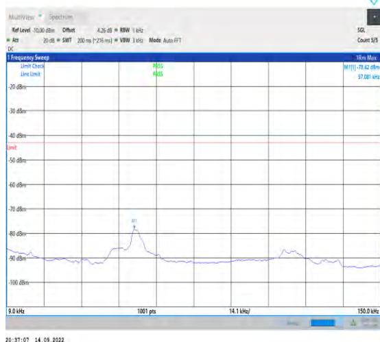
1-N78-3700-3800-PC2-30-100-L-1-DFT-PI2BPSK-In ner_1RB_Left-1@1-0.009-0.15-Ant1-0.06--78.42--4 3-PASS
