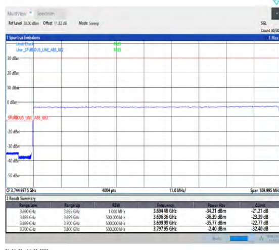
1-N78-3700-3800-PC2-30-100-L-6-CP-QPSK-Outer_Full-273@0-Ant1-1--PASS-see graph
