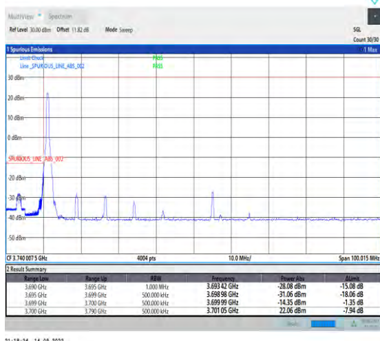
1-N78-3700-3800-PC2-30-90-L-1-DFT-PI2BPSK-Edge_1RB_Left-1@0-Ant1-1--PASS-see graph
