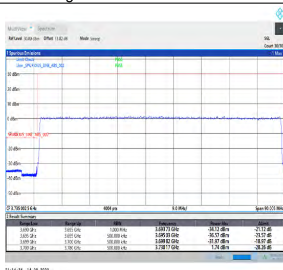
1-N78-3700-3800-PC2-30-80-L-3-DFT-PI2BPSK-Outer_Full-216@0-Ant1-1--PASS-see graph
