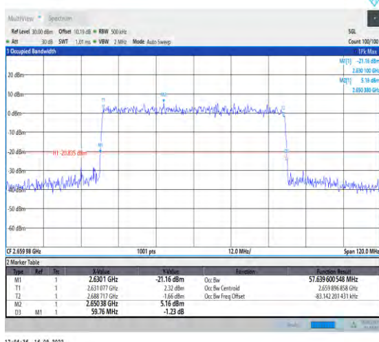
1-N41-PC2-30-60-H-9-CP-256QAM-Outer_Full-162 @0-Ant1-57.64-59.760-≤60-PASS
