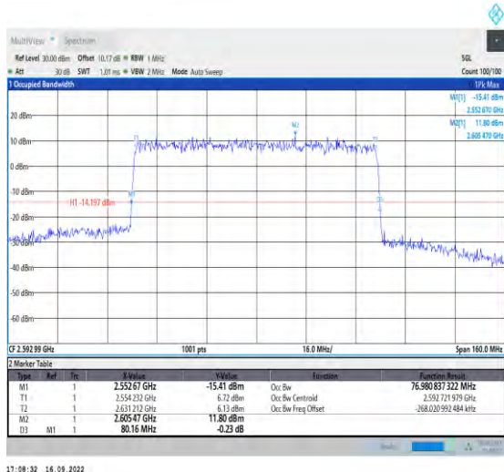
1-N41-PC2-30-80-M-3-DFT-16QAM-Outer_Full-216@0-Ant1-76.981-80.160-≤80-PASS
