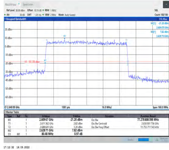
1-N41-PC2-30-80-H-9-CP-256QAM-Outer_Full-217 @0-Ant1-77.279-80.480-≤80-PASS
