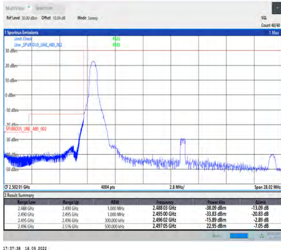
1-N41-PC2-30-20-L-1-DFT-PI2BPSK-Edge_1RB_Left-1@0-Ant1-1--PASS-see graph
