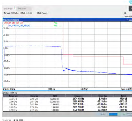
1-N41-PC2-30-30-H-6-CP-QPSK-Outer_Full-78@0-Ant1-1--PASS-see graph
