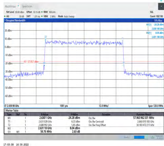
1-N41-PC2-30-60-H-6-CP-QPSK-Outer_Full-162@0-Ant1-57.964-59.760-≤60-PASS
