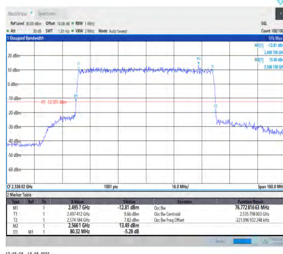
1-N41-PC2-30-80-L-1-DFT-QPSK-Outer_Full-216@0 -Ant1-76.773-80.320-≤80-PASS
