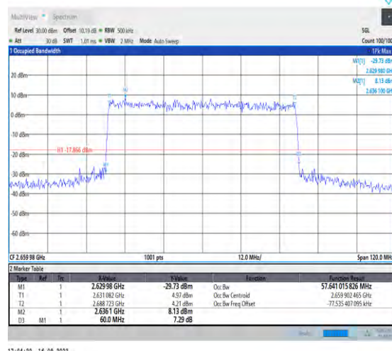
1-N41-PC2-30-60-H-8-CP-64QAM-Outer_Full-162@ 0-Ant1-57.641-60.000-≤60-PASS
