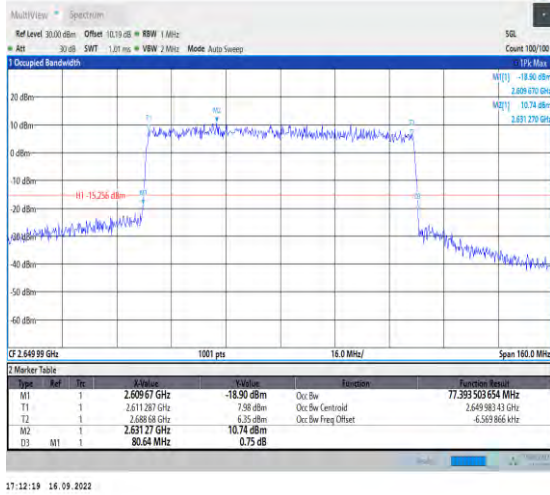
1-N41-PC2-30-80-H-8-CP-64QAM-Outer_Full-217@ 0-Ant1-77.394-80.640-≤80-PASS
