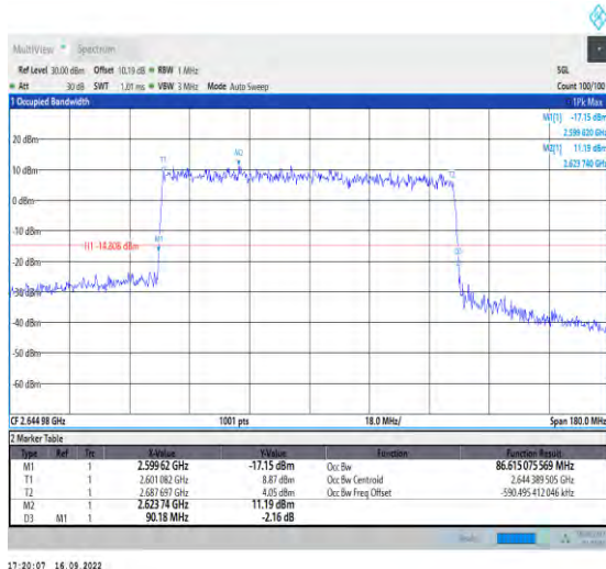
1-N41-PC2-30-90-H-3-DFT-16QAM-Outter_Full-243 @0-Ant1-86.615-90.180-≤90-PASS
