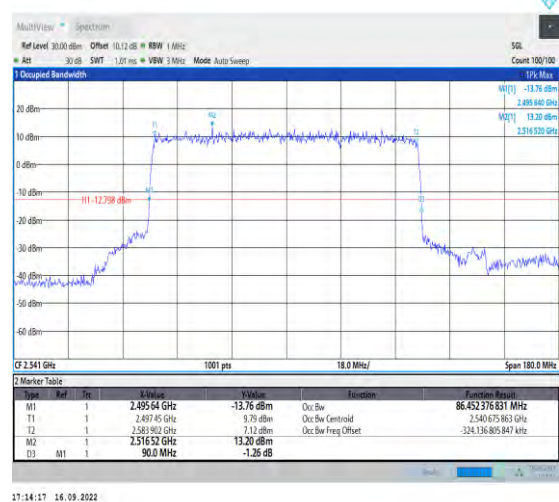
1-N41-PC2-30-90-L-2-DFT-PI2BPSK-Outer_Full-243 @0-Ant1-86.452-90.000-≤90-PASS
