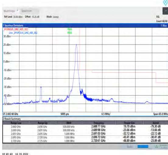
1-N41-PC2-30-30-H-5-CP-QPSK-Edge_1RB_Right-1@77-Ant1-1--PASS-see graph
