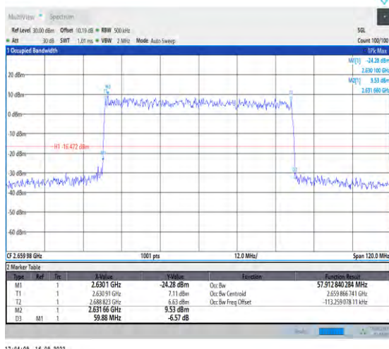
1-N41-PC2-30-60-H-7-CP-16QAM-Outer_Full-162@ 0-Ant1-57.913-59.880-≤60-PASS
