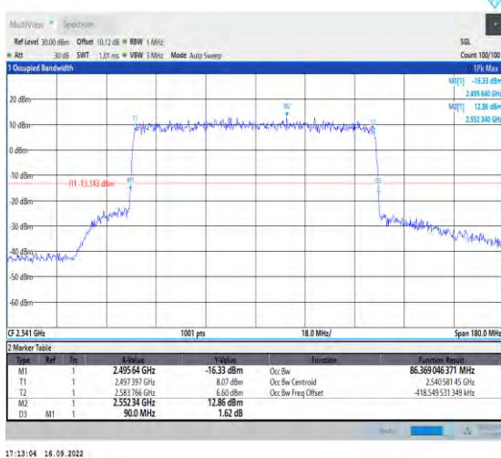
1-N41-PC2-30-90-L-1-DFT-QPSK-Outer_Full-243@ 0-Ant1-86.369-90.000-≤90-PASS
