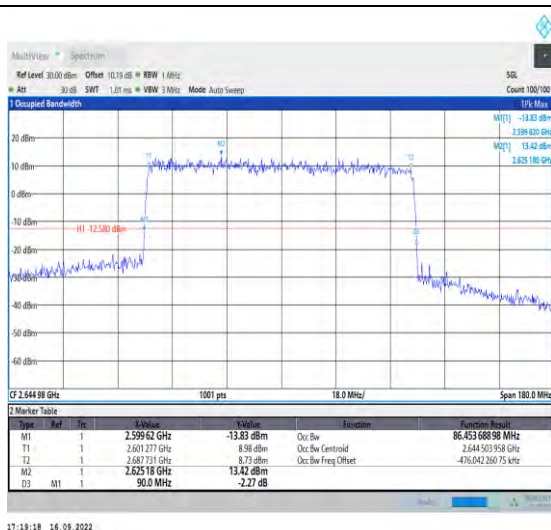
1-N41-PC2-30-90-H-1-DFT-QPSK-Outter_Full-243@ 0-Ant1-86.454-90.000-≤90-PASS
