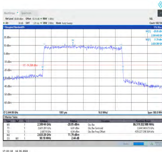
1-N41-PC2-30-90-H-4-DFT-64QAM-Outter_Full-243 @0-Ant1-86.519-90.180-≤90-PASS
