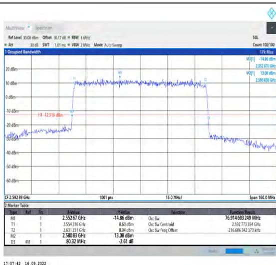
1-N41-PC2-30-80-M-1-DFT-QPSK-Outer_Full-216@ 0-Ant1-76.915-80.320-≤80-PASS
