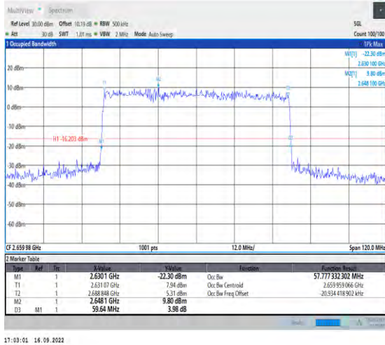
1-N41-PC2-30-60-H-3-DFT-16QAM-Outer_Full-162 @0-Ant1-57.777-59.640-≤60-PASS
