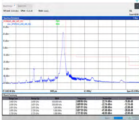
1-N41-PC2-30-30-H-2-DFT-PI2BPSK-Edge_1RB_Right-t-1@77-Ant1-1--PASS-see graph
