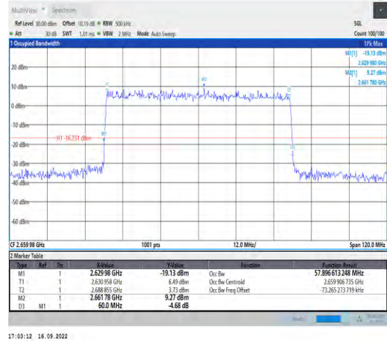
1-N41-PC2-30-60-H-4-DFT-64QAM-Outer_Full-162 @0-Ant1-57.897-60.000-≤60-PASS
