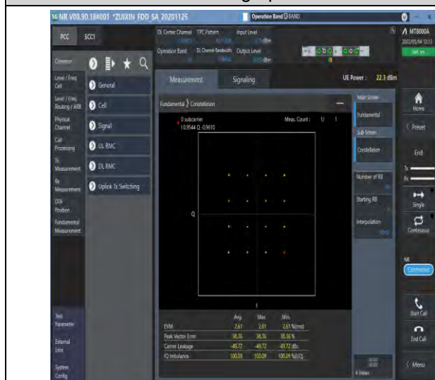
1-N14-PC3-15-10-M-3-DFT-16QAM-Outter_Full-50@0 -Ant1-see graph-PASS
