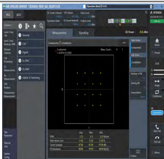
1-N14-PC3-15-10-M-7-CP-16QAM-Outer_Full-52@0-Ant1-see graph-PASS
