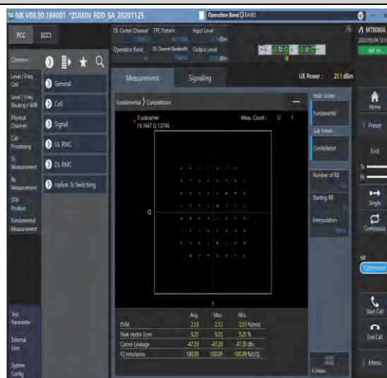
1-N14-PC3-15-10-M-8-CP-64QAM-Outer_Full-52@0-Ant1-see graph-PASS
