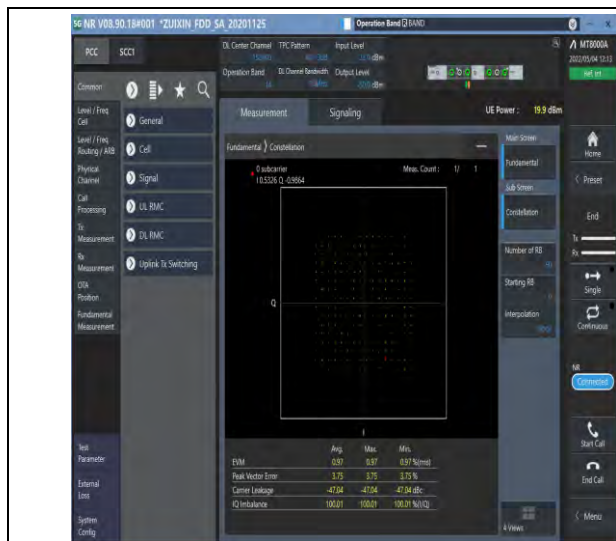
1-N14-PC3-15-10-M-5-DFT-256QAM-Outer_Full-50@0-Ant1-see graph-PASS
