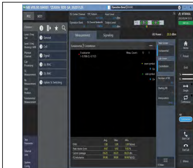
1-N14-PC3-15-10-M-1-DFT-PI2BPSK-Outter_Full-50@ 0-Ant1-see graph-PASS
