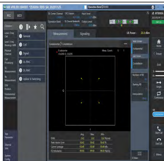
1-N14-PC3-15-10-M-2-DFT-QPSK-Outter_Full-50@0 -Ant1-see graph-PASS
