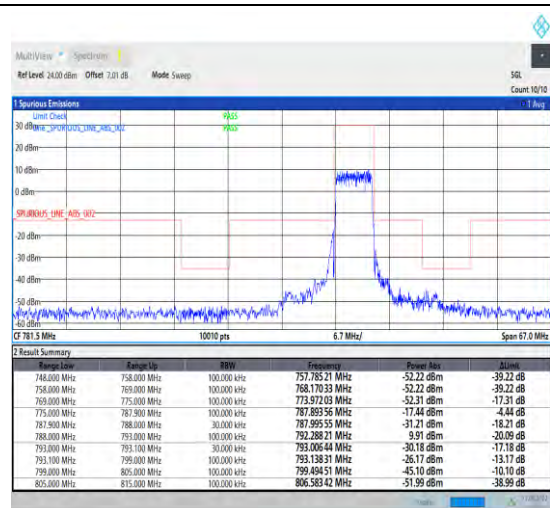
1-N14-PC3-15-5-L-3-DFT-PI2BPSK-Outer_Full-25 @0-Ant1-1--PASS-see graph
