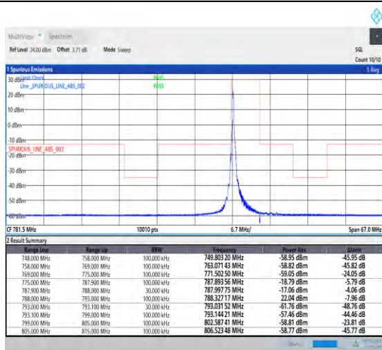
1-N14-PC3-15-5-L-1-DFT-PI2BPSK-Edge_1RB_Left-1 @0-Ant1-1--PASS-see graph
