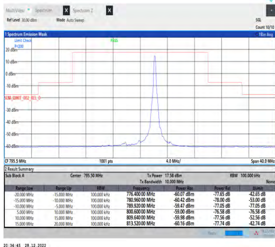
1-N14-PC3-15-5-H-2-DFT-PI2BPSK-Edge_1RB_Right-1 @24-Ant1-1--PASS-see graph
