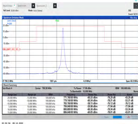
1-N14-PC3-15-5-L-1-DFT-PI2BPSK-Edge_1RB_Left-1 @0-Ant1-1--PASS-see graph
