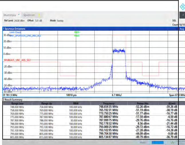
1-N14-PC3-15-5-L-3-DFT-PI2BPSK-Outer_Full-25 @0-Ant1-1--PASS-see graph
