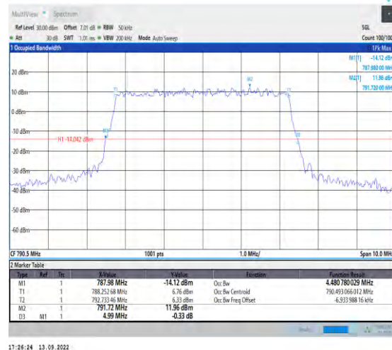
1-N14-PC3-15-5-L-4-DFT-64QAM-Outet_Full-25@0-Ant1-4.481-4.990-≤5-PASS
