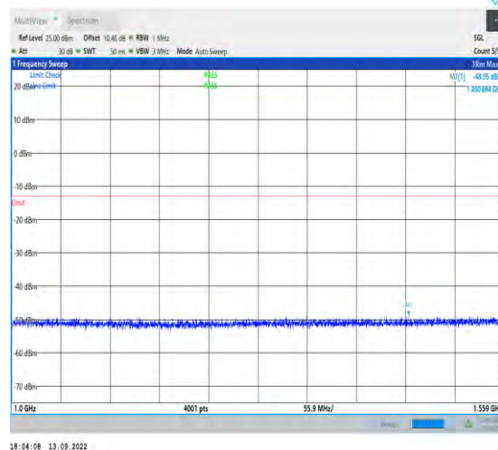
1-N14-PC3-15-10-M-1-DFT-PI2BPSK-Inner_1RB_Lef t-1@1-1000-1559-Ant1-1546.14--48.95--13-PASS
