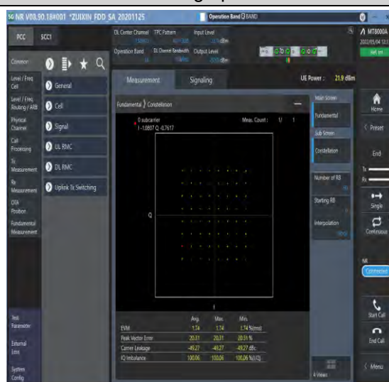
1-N14-PC3-15-10-M-4-DFT-64QAM-Outter_Full-50@0 0-Ant1-see graph-PASS
