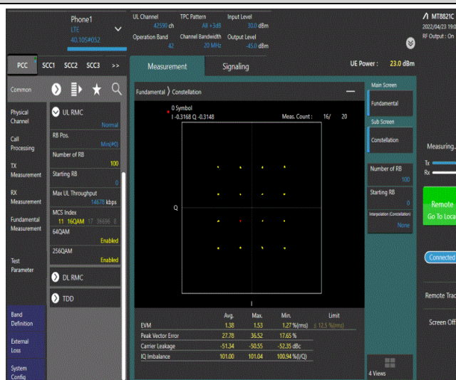
Band42-20MHz-16QAM-42590-100RB#0
