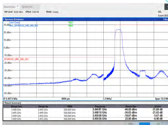
Band42-5MHz-QPSK-42115-25RB#0
