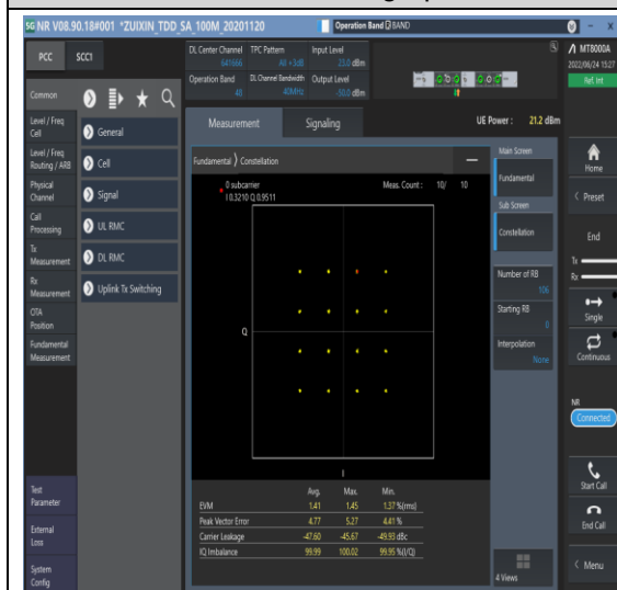
1-N48-PC3-30-40-M-7-CP-16QAM-Out_Ful-I-106@0-Ant1-see graph-PASS
