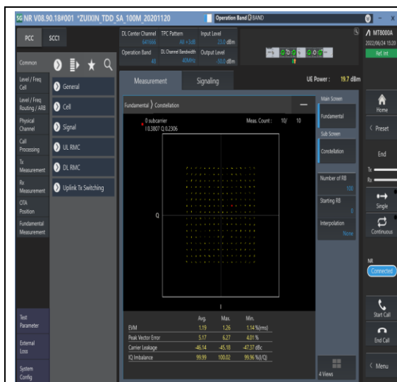
1-N48-PC3-30-40-M-5-DFT-256QAM-Out_Full-100@0-Ant1-see graph-PASS
