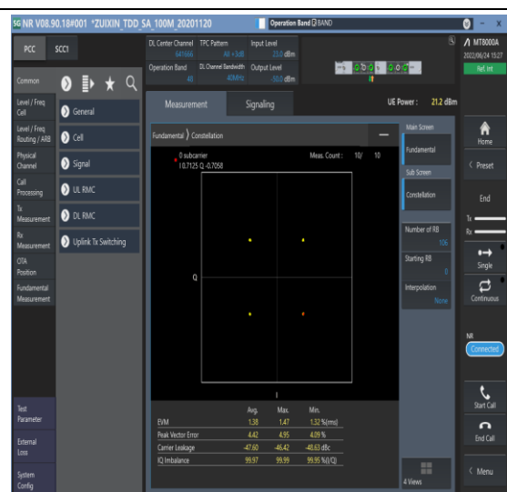
1-N48-PC3-30-40-M-6-CP-QPSK-Out_Full-106@0-Ant1-see graph-PASS
