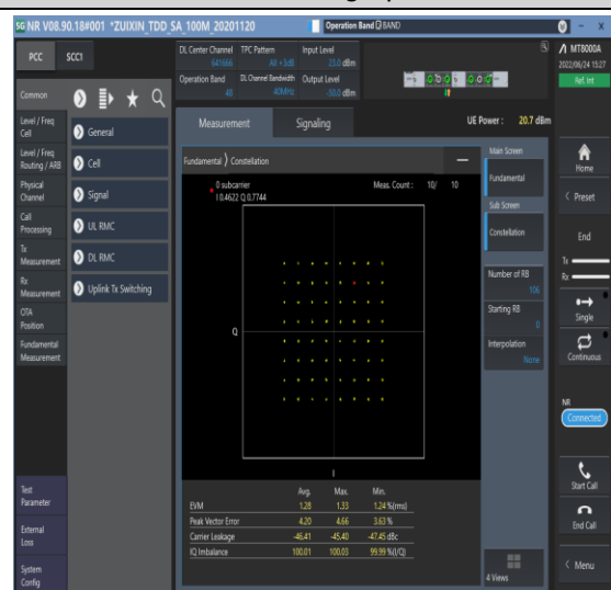
1-N48-PC3-30-40-M-8-CP-64QAM-Out_Ful-I-106@0-Ant1-see graph-PASS
