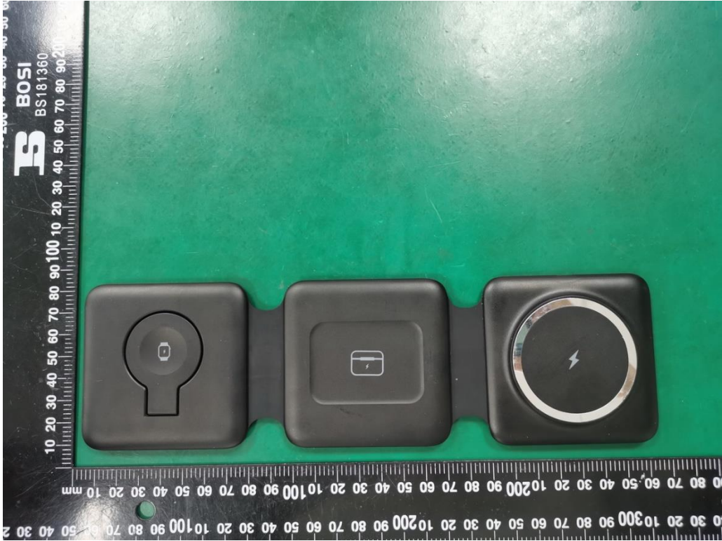
External Photo FCC ID: 2A8QNWZC-CW340
