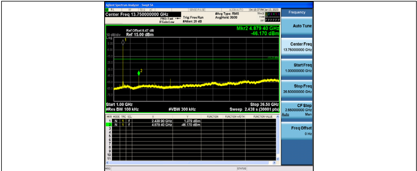
BLE_2M_Ant1_2480_0~Reference
