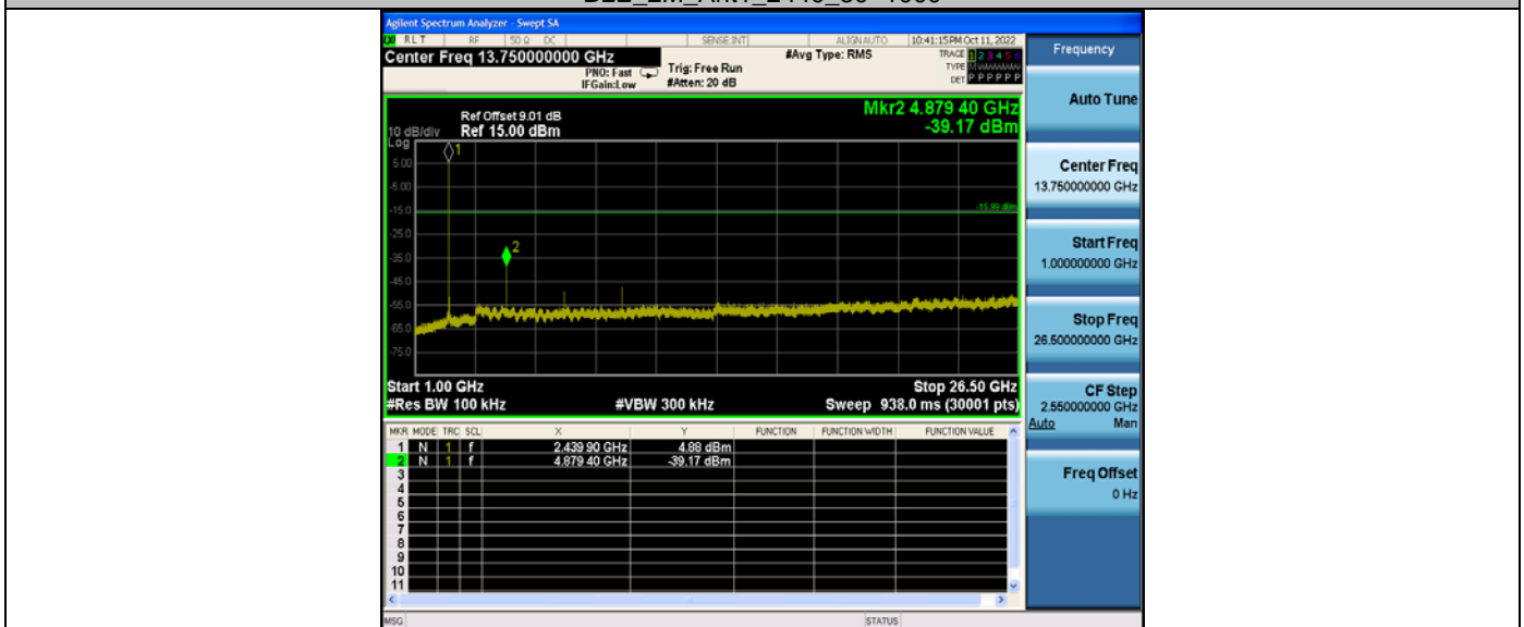
BLE_2M_Ant1_2440_1000~26500
