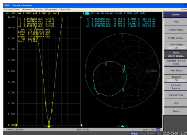
Fig.1 驻波比 VSWR
