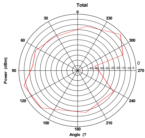
XY Plane at f = 0.434\text{GHz}
