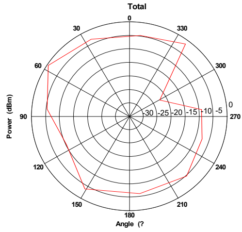
XZ Plane at f = 0.434\text{GHz}
