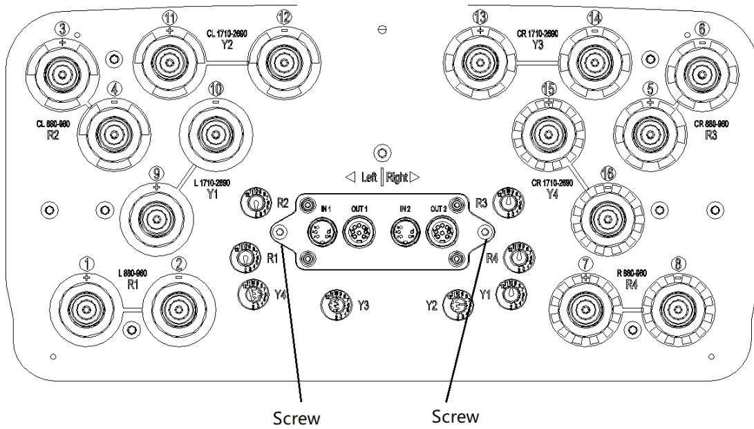
Figure 3 MIRCU Installation
