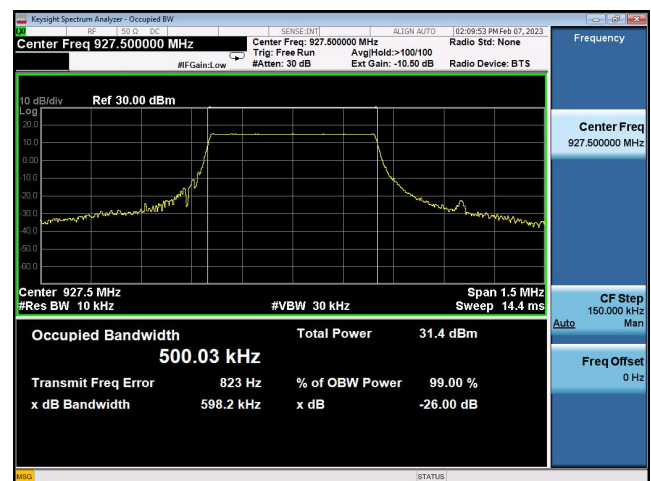
99% Bandwidth: 927.5MHz
