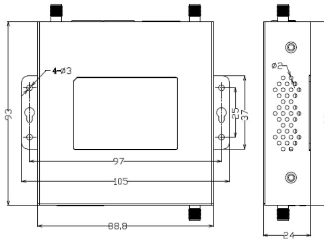
DIN Rail Style Router Dimension
