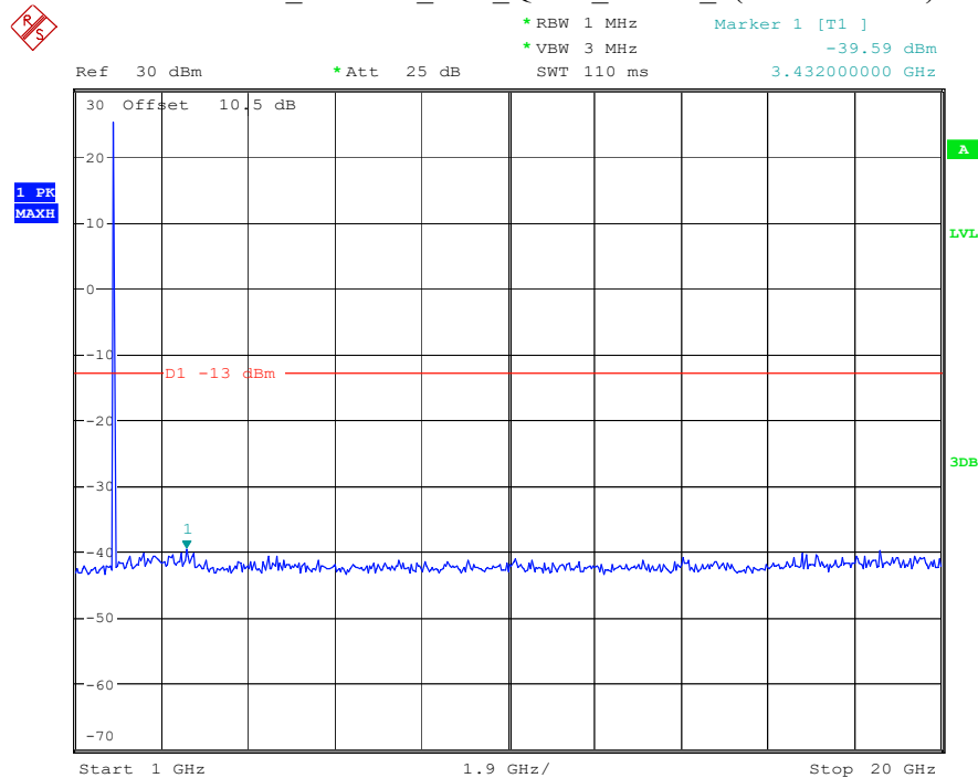
Band 2_1.4 MHz_Low_QPSK_RB6#0_2(1GHz-20GHz)
