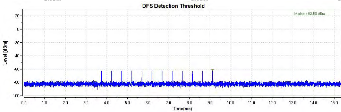
Radar Singal 4
