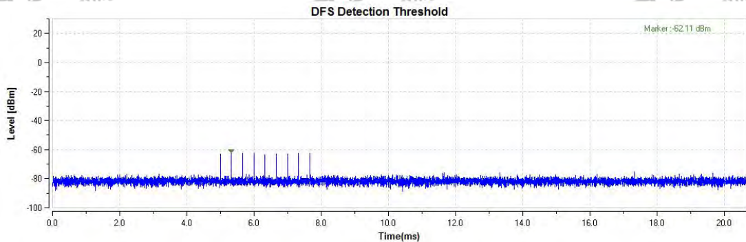
Radar Singal 6
