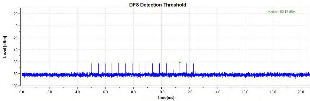
Radar Singal 3
