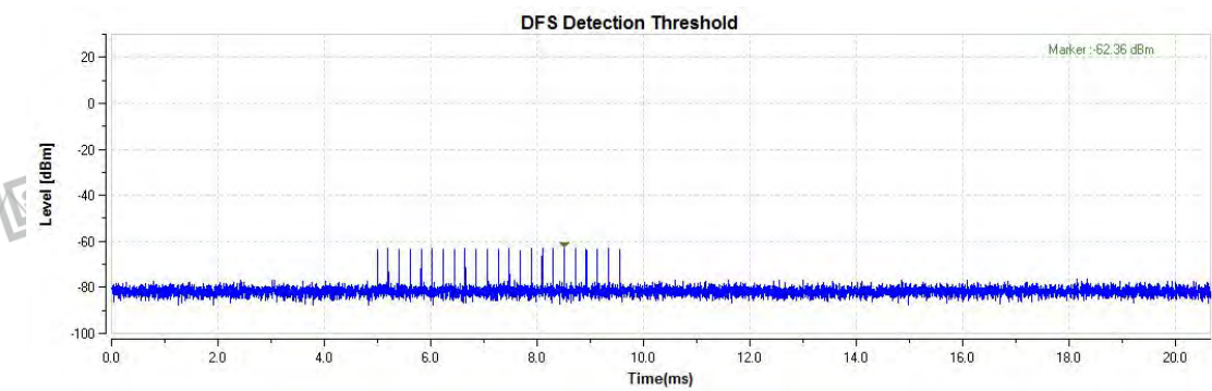
Radar Singal 2
