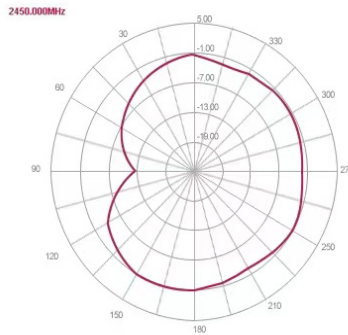
Passive Test For wifi
