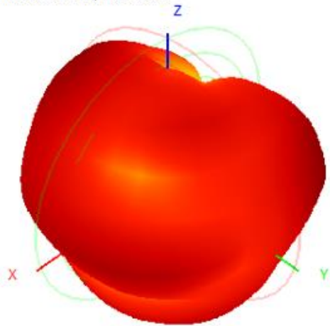
2402.0MHz H+V, Eff: 45.6%
