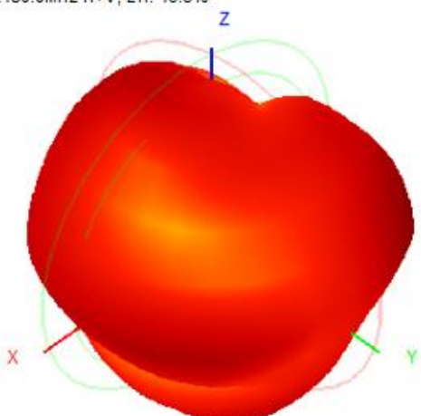
2480.0MHz H+V, Eff: 46.3%
