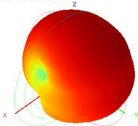
2440.0MHz H+V, Eff: 46.7%
