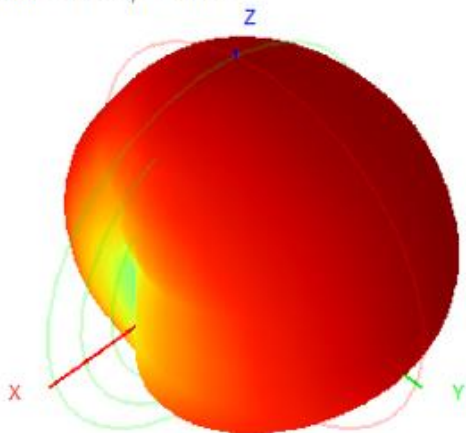
2480.0MHz H+V, Eff: 49.2%
