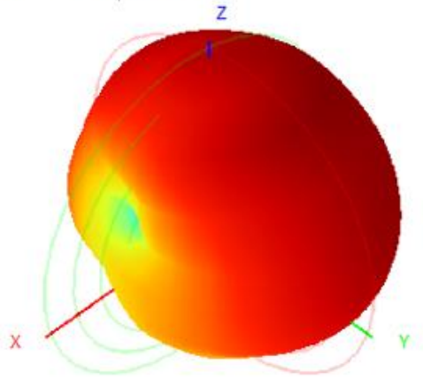
2402.0MHz H+V, Eff: 42.2%
