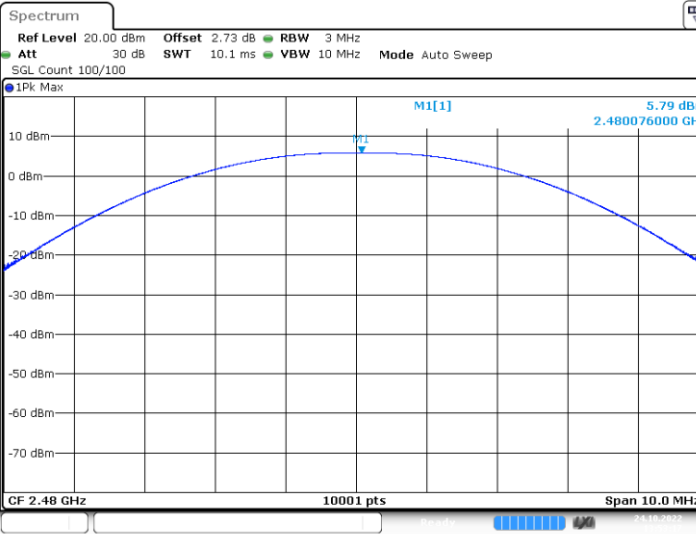
Channel 39 (2480MHz)
