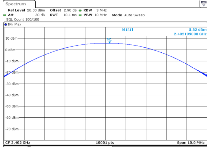
Channel 0 (2402MHz)
