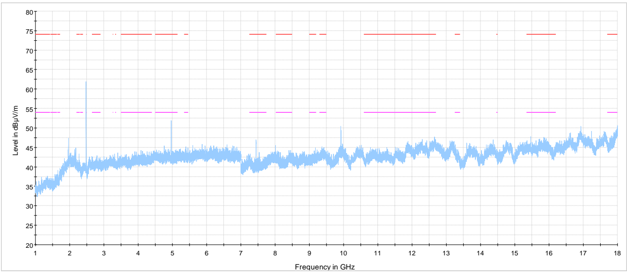
PRJ0023932 RE 1-18 GHz, FET, ch. 26 Preview Result 1-PK+ FCC 15.209 and RSS-Gen Restricted bands peak limits FCC 15.209 and RSS-Gen Restricted bands average limits
