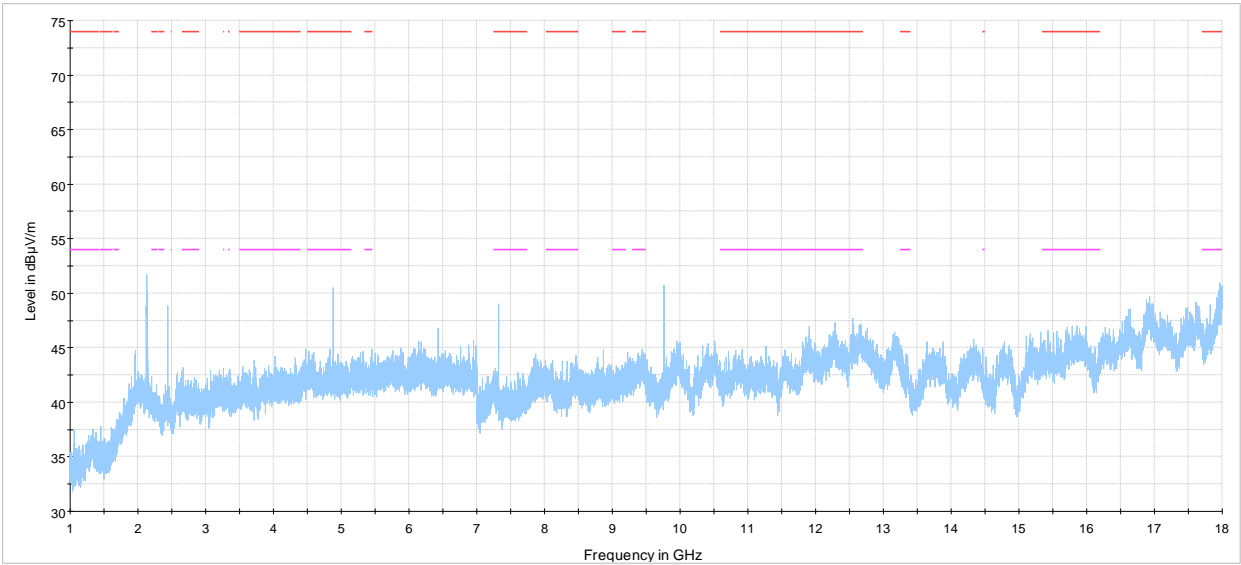
PRJ0023932 RE 1-18 GHz ch. 18 Preview Result 1-PK+ FCC 15.209 and RSS-Gen Restricted bands peak limits FCC 15.209 and RSS-Gen Restricted bands average limits
