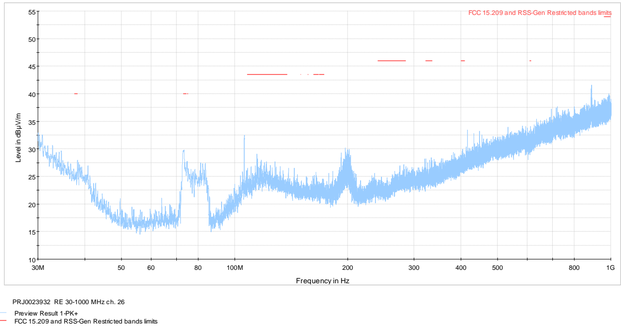
Figure 8.1-3: Radiated spurious emissions 30-1000 MHz high channel
