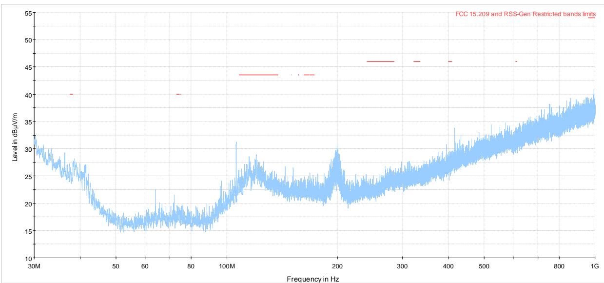
Figure 8.1-1: Radiated spurious emissions 30-1000 MHz low channel
