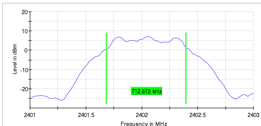
6 dB Bandwidth
