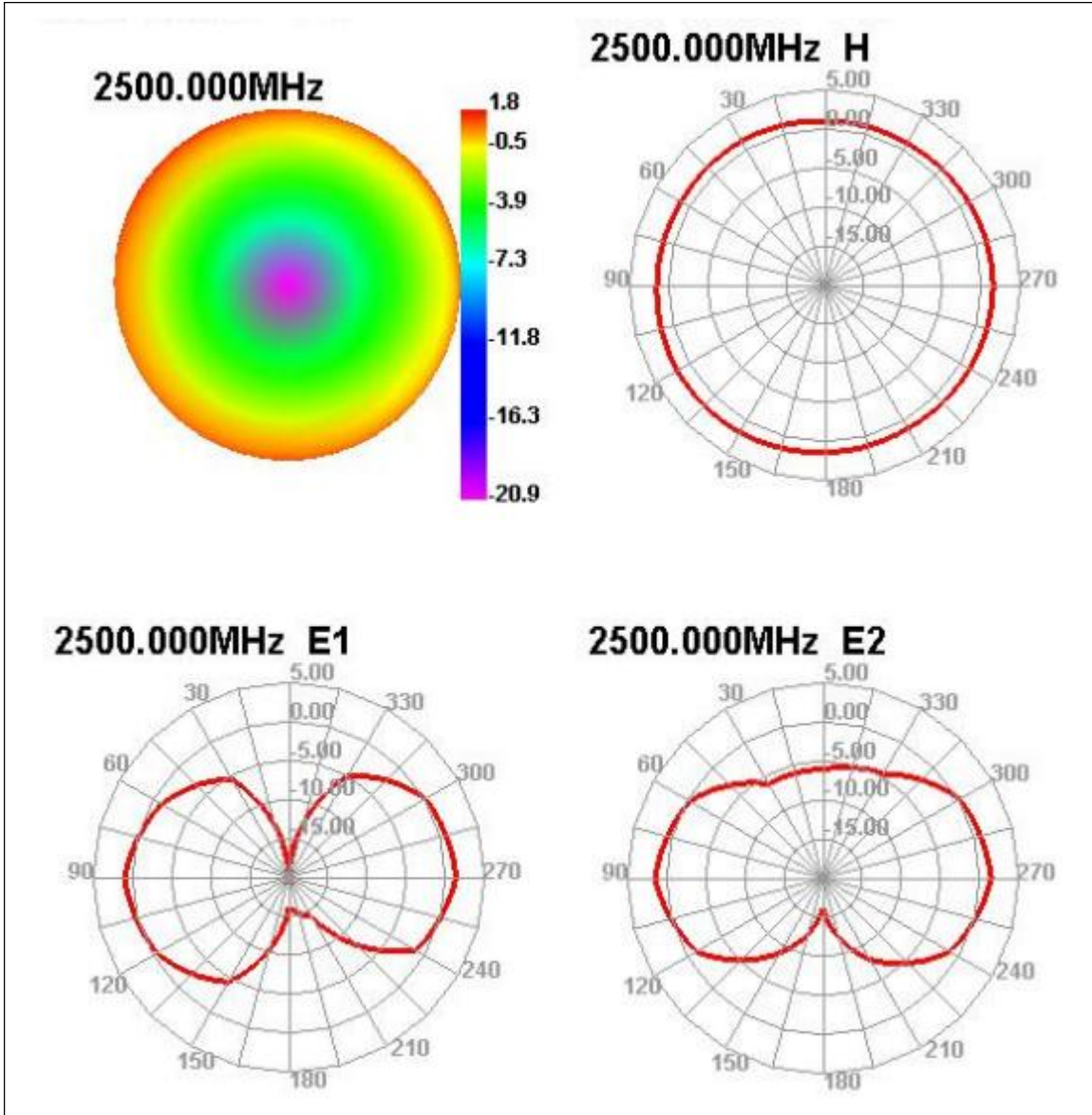
Antenna Pattern/Measurement data
