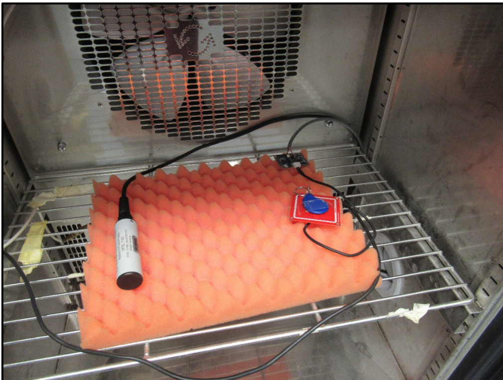
Photo 6 Test Setup - Frequency Stability (Temperature & Voltage Variation)
