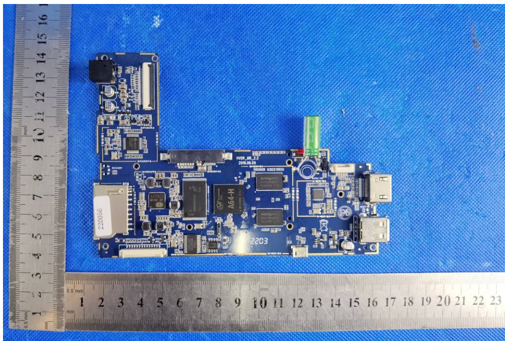
INTERNAL VIEW OF EUT(FIGURE 2)
