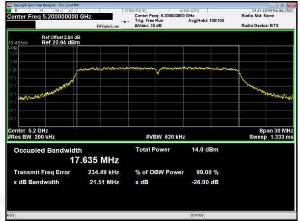
(802.11 n20) 26dB Bandwidth plot on channel 40
