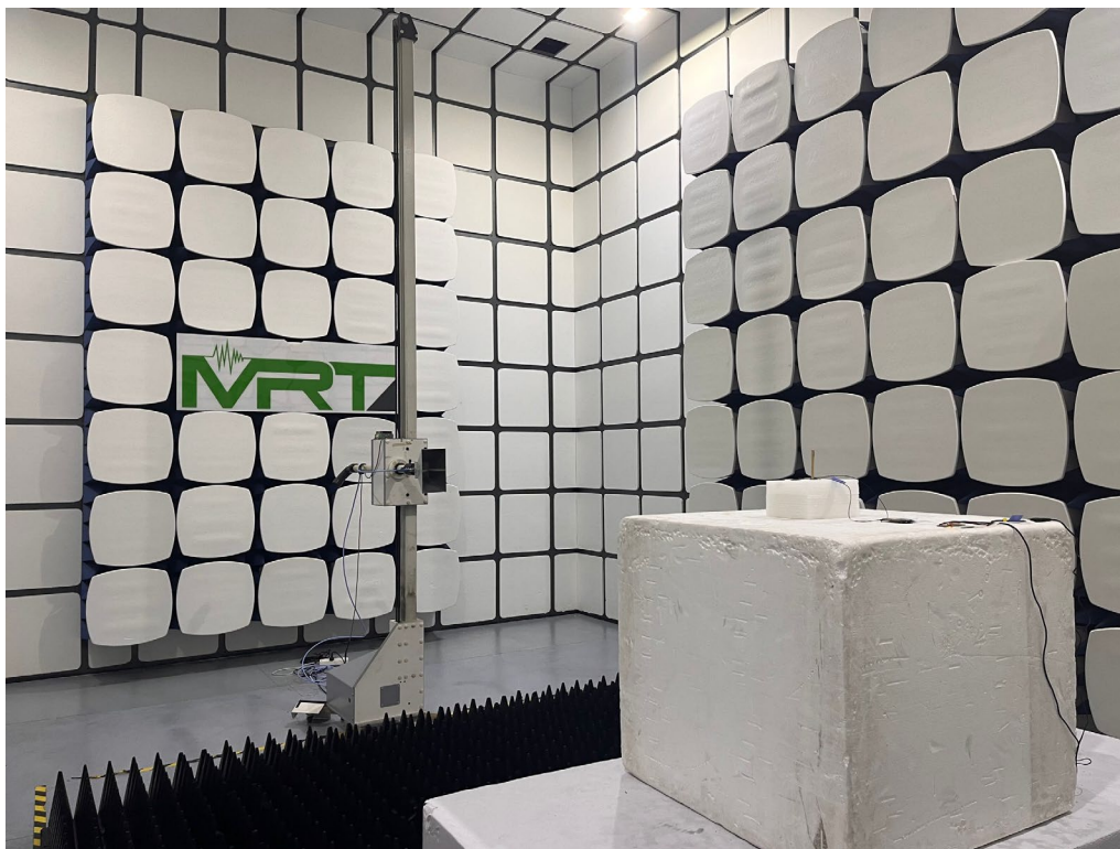
Description: Radiated Restricted Band Edge Test Setup for Ant 1
