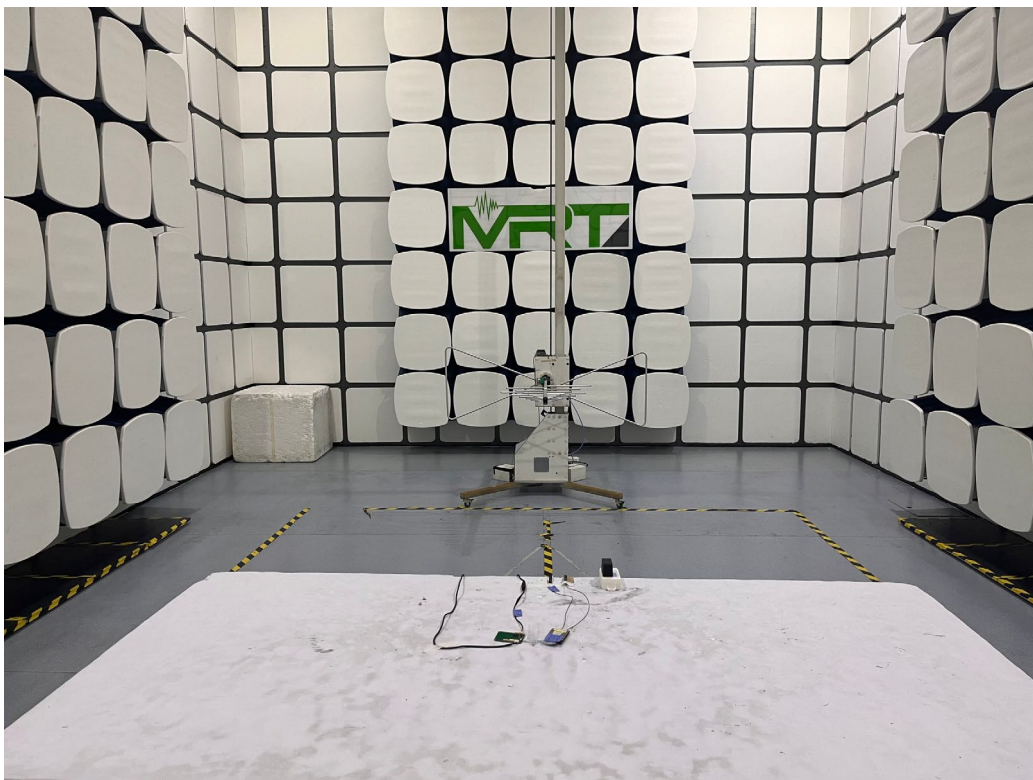
Description: Radiated Spurious Emission Test Setup for Ant 1 Above 1GHz
