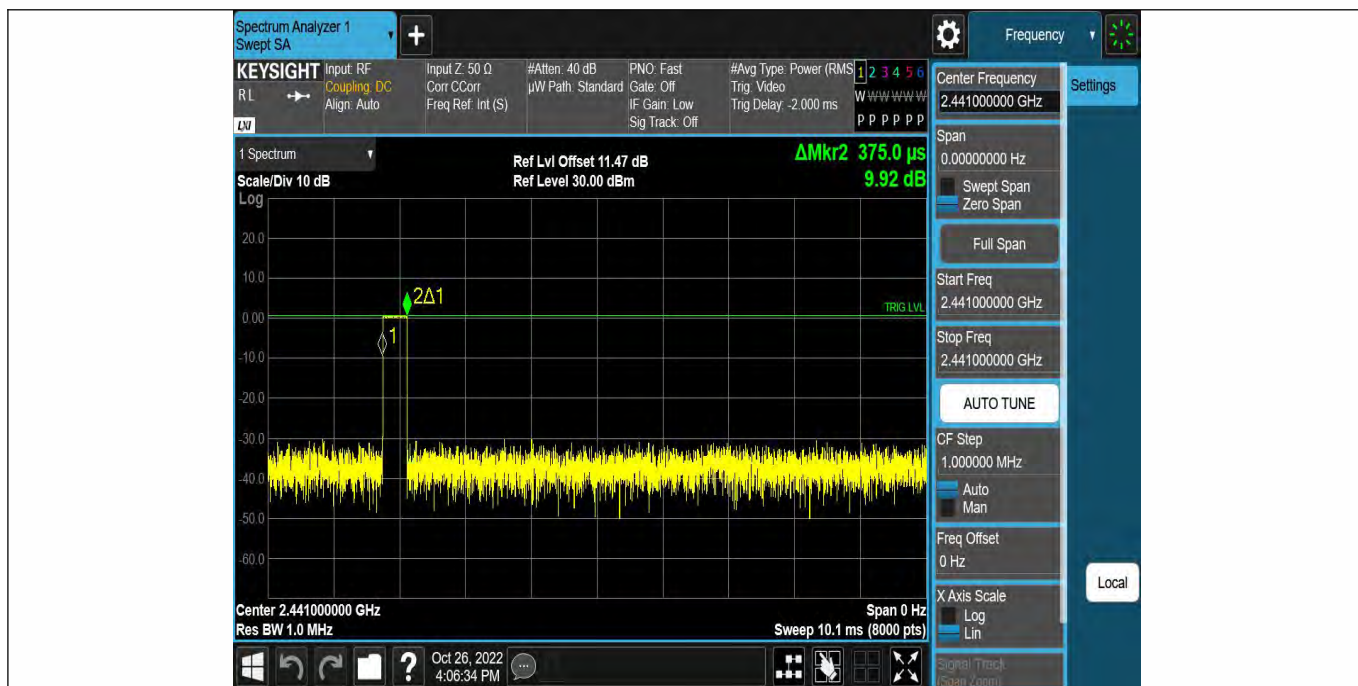
DH1-Ant1-Hop-0.375-320
