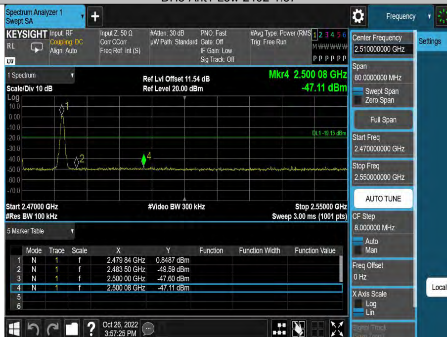
DH5-Ant1-High-2480-0.85
