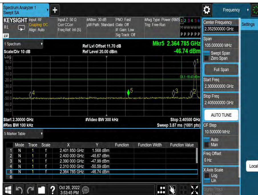
DH5-Ant1-Low-2402-1.57
