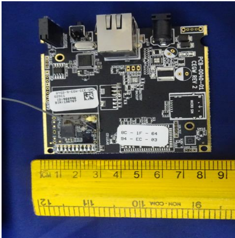
PCB_Dimensional view
