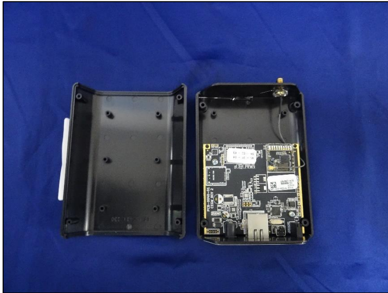
Open enclosure
