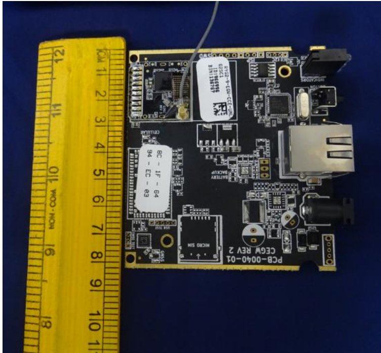
PCB_Dimensional view
