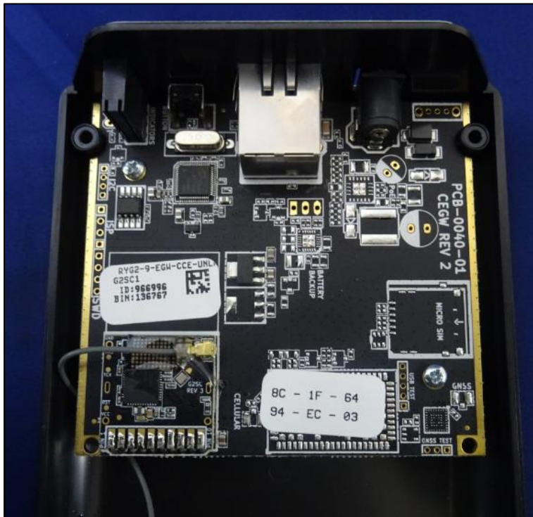
PCB_front view
