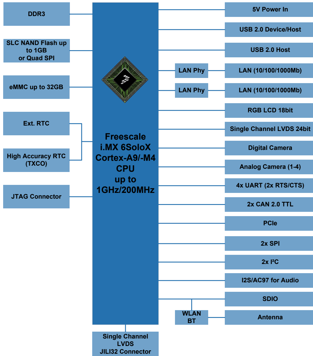
Figure 1: Block diagram
