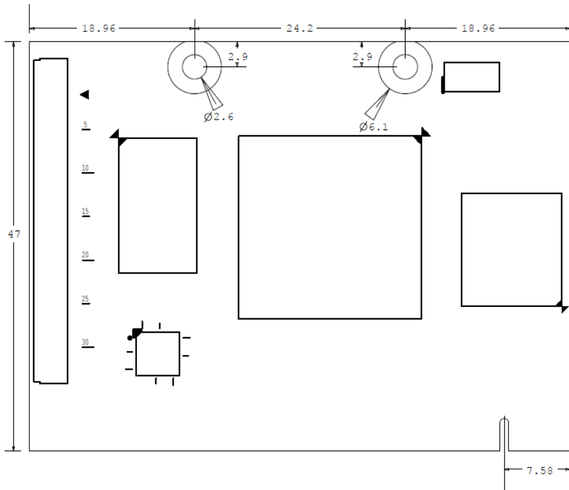
Figure 2: Mechanical dimensions
