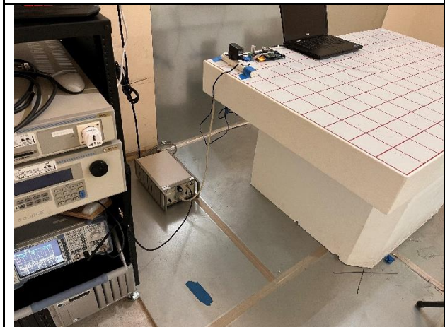
Conducted Emission Test Front View
