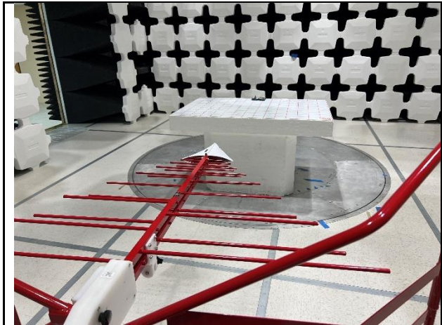
Radiated Emission Test below 30MHz Front View
