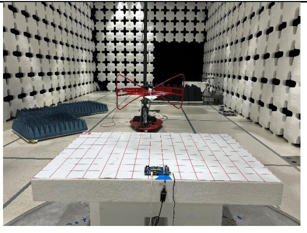
Radiated Emission Test below 30GHz Rear View
