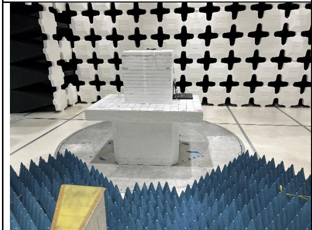
Radiated Emission Test below 1GHz Front View
