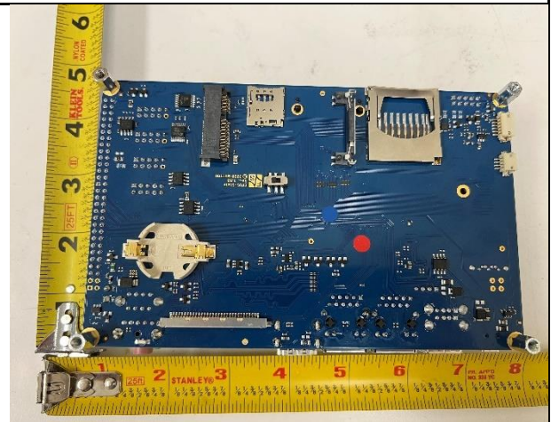
Interface board Bottom view
