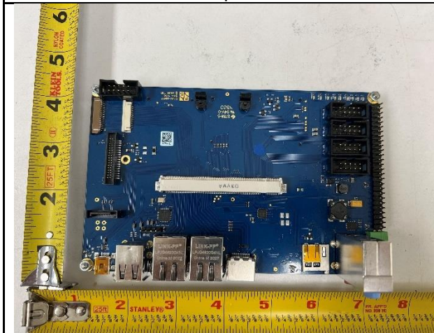
Interface board Top view
