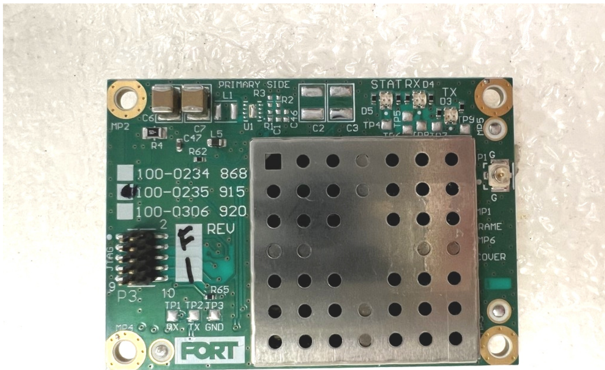
EUT/ RF Module PCB Primary Side
