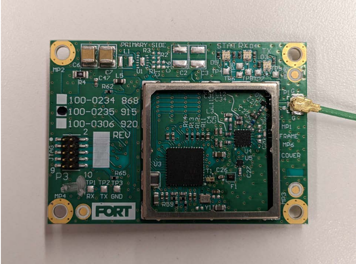
EUT/ RF Module with shielding cover removed
