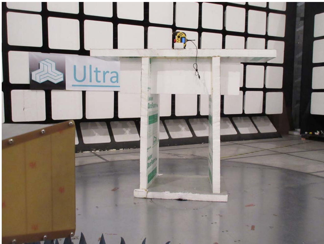
Radiated Emissions at 3 m EUT with 1.6 dBi Linx Technologies Inc ¼ wave whip, straight antenna, Orthogonal Position 3
