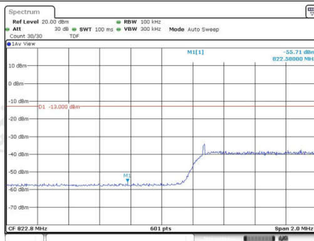
Band26-5MHz-QPSK-26803-1RB#0
