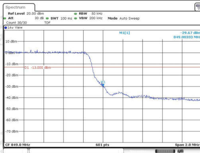
Band26-3MHz-16QAM-27025-15RB#0
