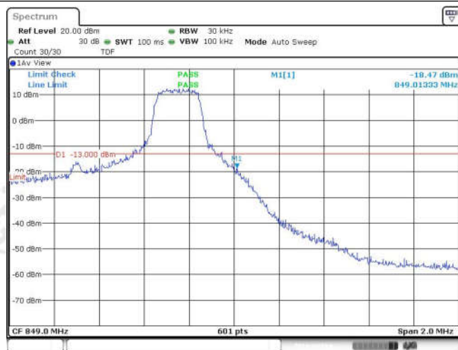
Band26-1.4MHz-16QAM-27033-6RB#0
