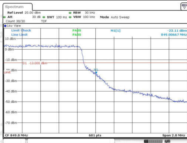
Band26-1.4MHz-16QAM-27033-6RB#0
