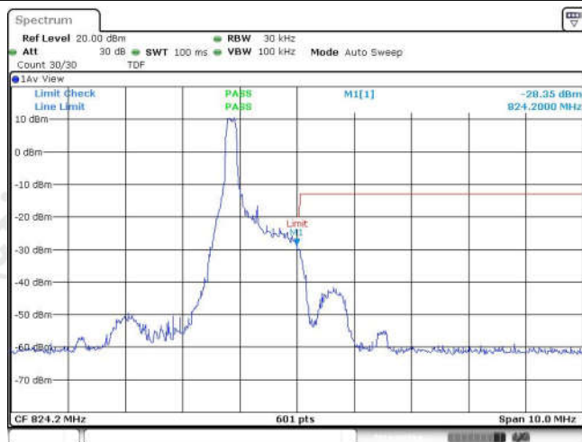
Band26-1.4MHz-16QAM-26785-1RB#0
