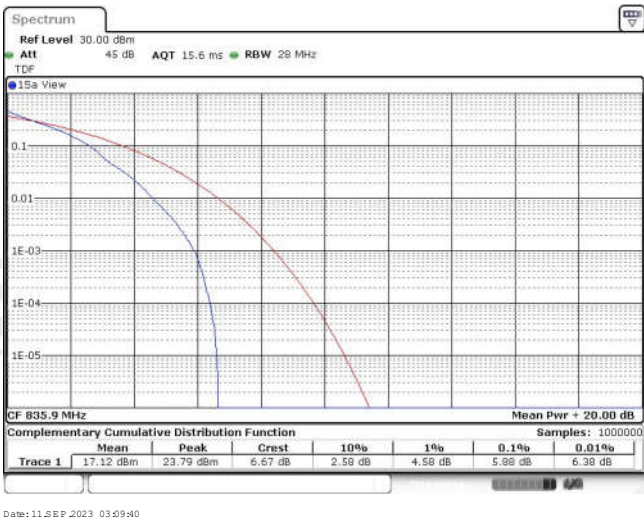
Band26-10MHz-QPSK-26909-50RB#0
