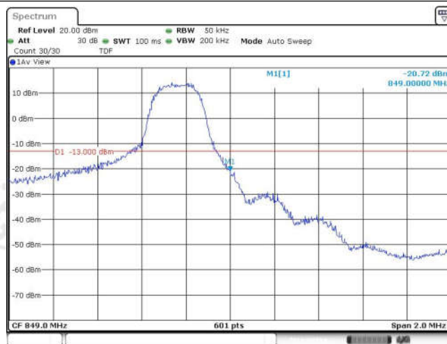
Band26-3MHz-16QAM-27025-15RB#0
