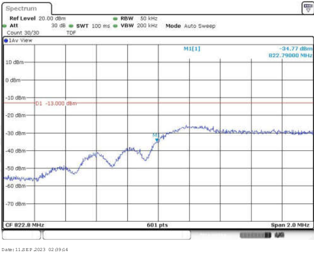
Band26-3MHz-16QAM-26793-15RB#0
