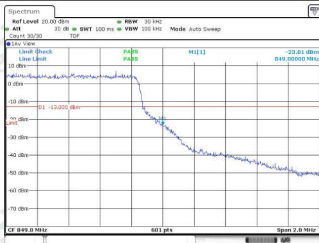
Band26-1.4MHz-QPSK-27033-6RB#0
