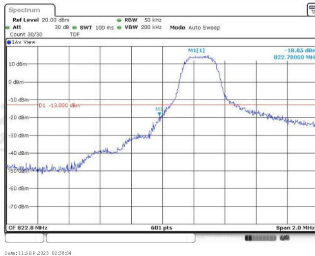
Band26-3MHz-16QAM-26793-1RB#14
