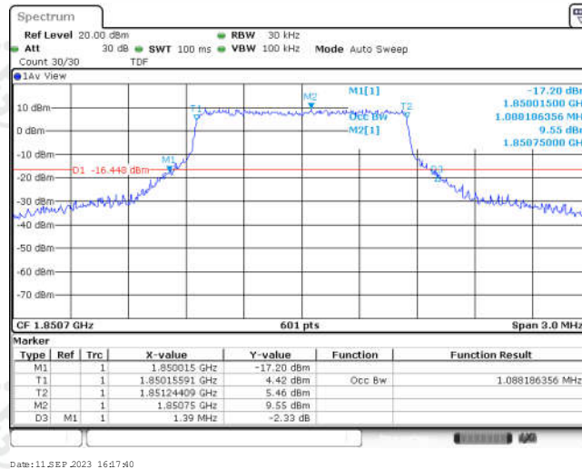
Band25-1.4MHz-16QAM-26365-6RB#0-1.088
