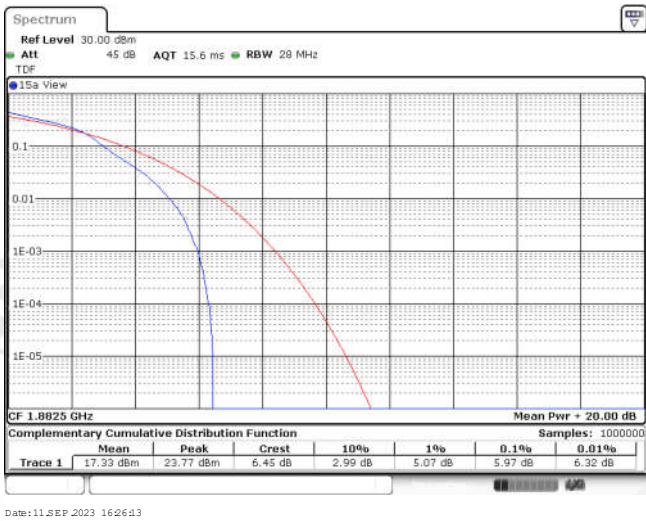
Band25-1.4MHz-16QAM-26365-6RB#0
