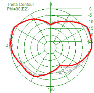
Efficiency: 86.7%
