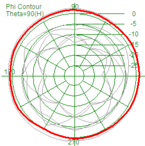
Gain (Peak): 1.87 dBi
