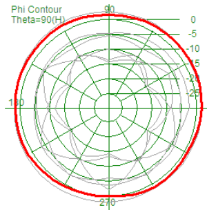
Gain (Peak): 0.87 dBi
