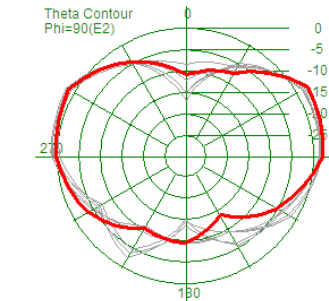
Efficiency: 82.2%
