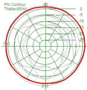
Gain (Peak): 2.01 dBi
