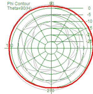
Gain (Peak): 1.02 dBi
