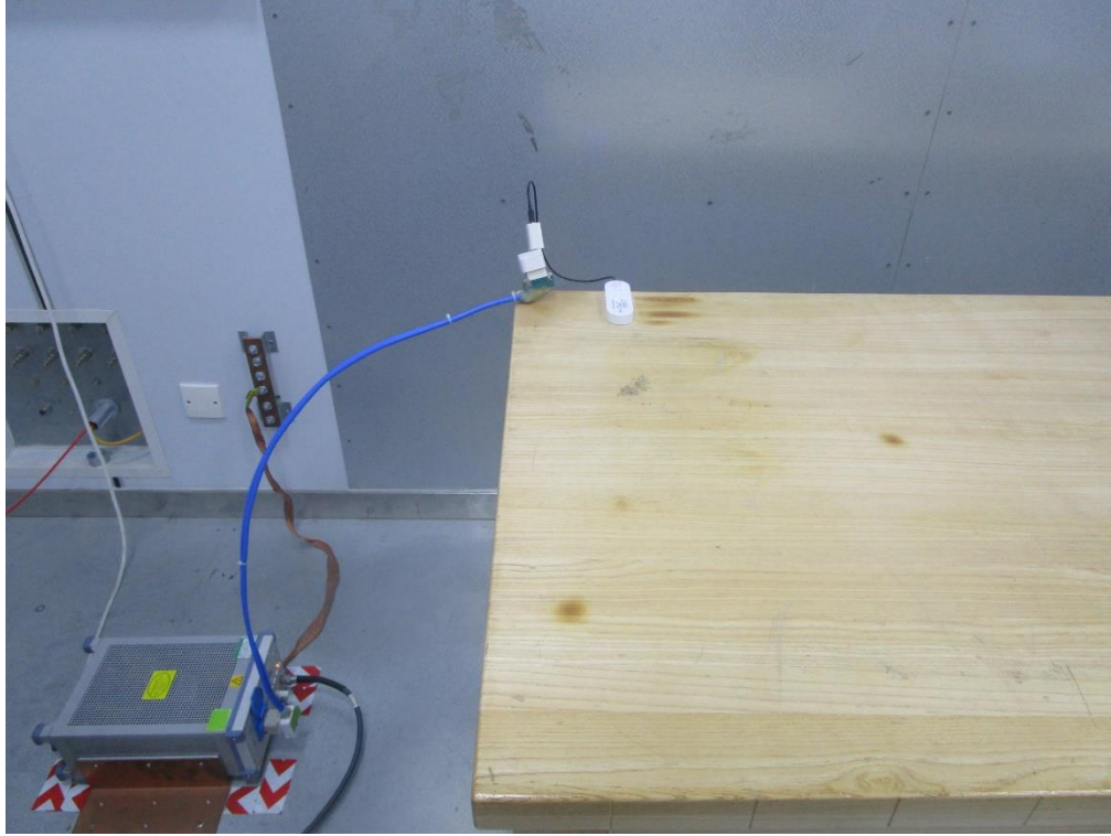
9KHz-30MHz Radiated Emission Test Setup Photo
