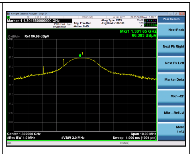
3 rd harmonic
