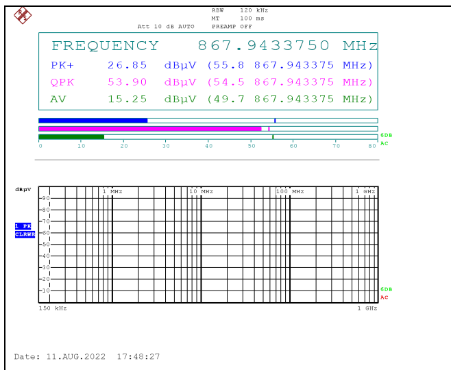
2 nd harmonic
