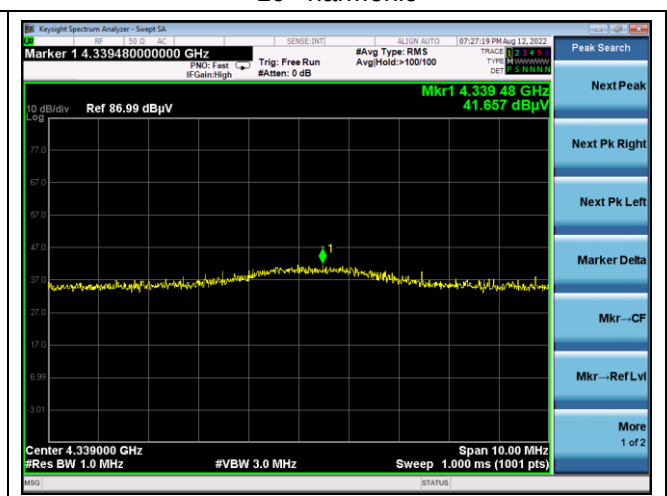
10 th harmonic
