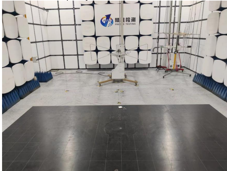
Radiated Spurious Emissions Test Frequency From Below 30MHz-1000MHz
