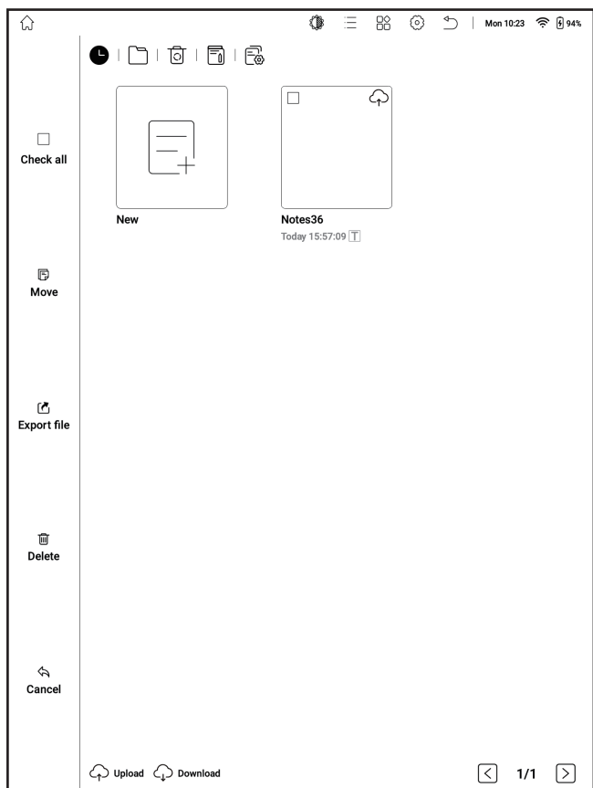
Multi-select
