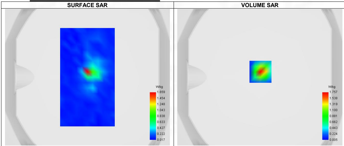
Maximum location: X=1.00, Y=8.00 ; SAR Peak: 3.13 W/kg
