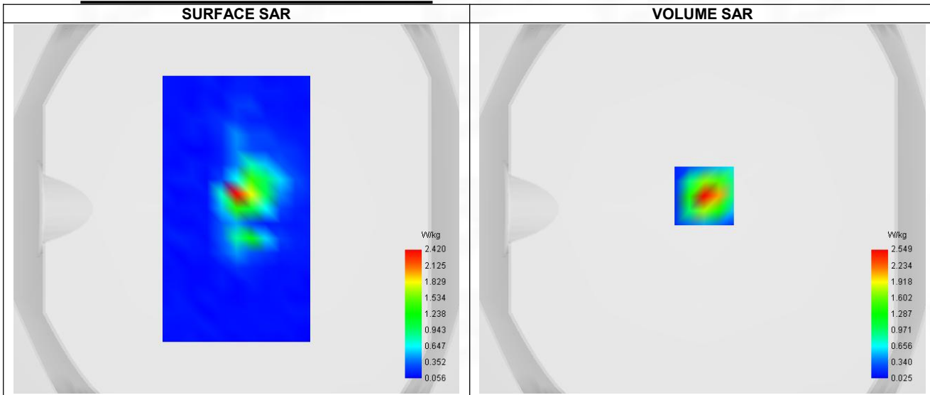
Maximum location: X=1.00, Y=7.00 ; SAR Peak: 4.63 W/kg
