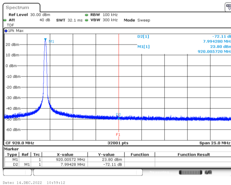
Graph 10: Upper Band Edge Plot (Antenna-Port Conducted)
