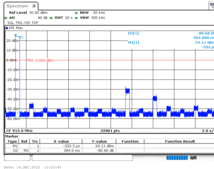
Graph 6: Channel Occupancy Showing a Single Hit in 20 Seconds
