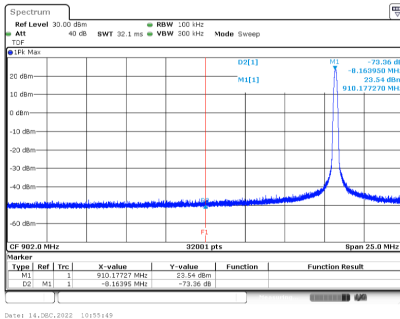
Graph 9: Lower Band Edge Plot (Antenna-Port Conducted)
