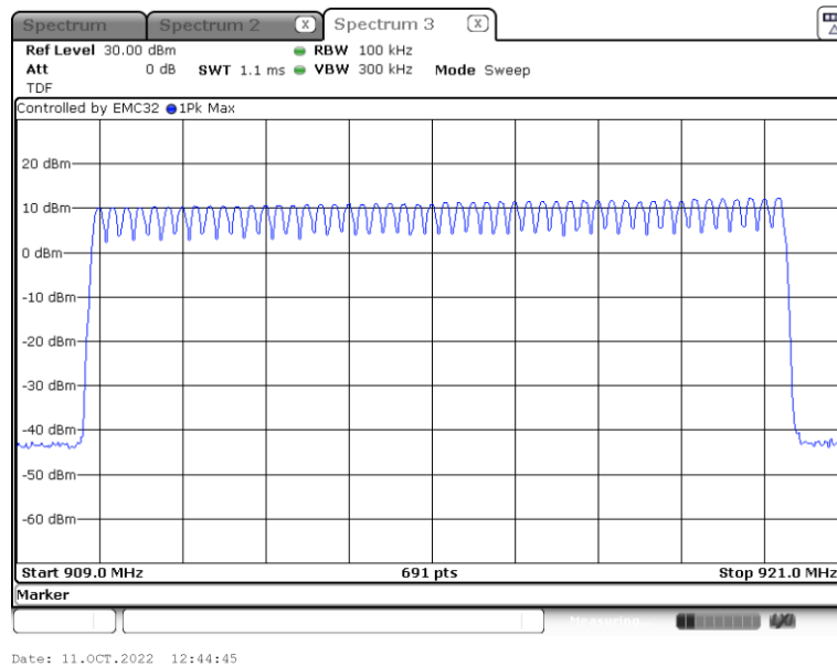
Graph 8: Radiated Plot Showing all 50 Hopping Frequencies within the Authorized Band
