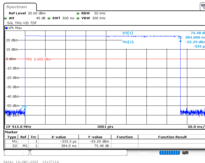
Graph 7: Channel Occupancy Showing a Channel Dwell Time of 384 ms
