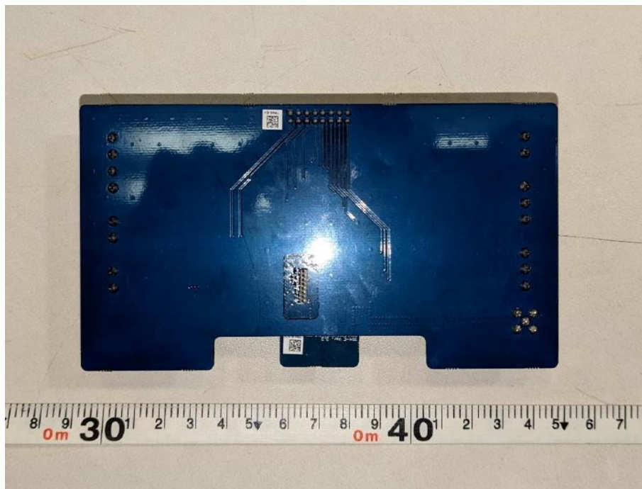
Photograph 4 – Back View of EUT with RF Shield, Mounted on Evaluation Board for Testing
