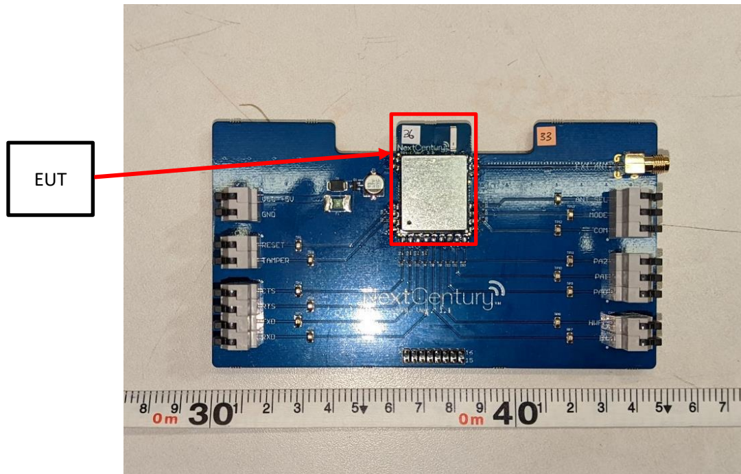
Photograph 3 – Front View of EUT with RF Shield, Mounted on Evaluation Board for Testing
