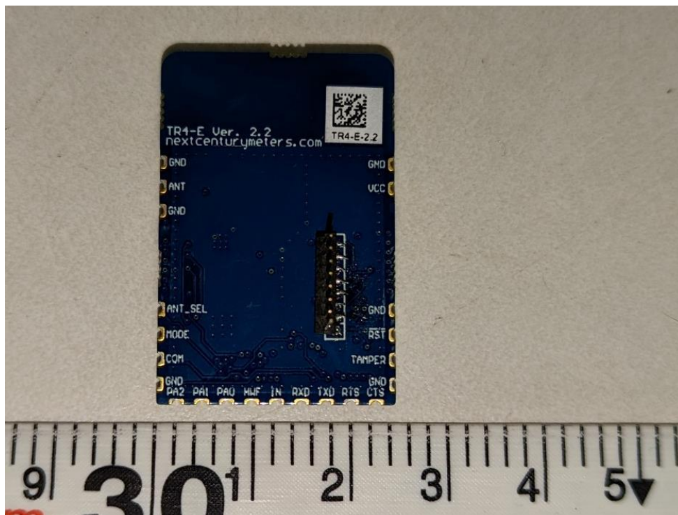
Photograph 2 – Back View of the EUT
