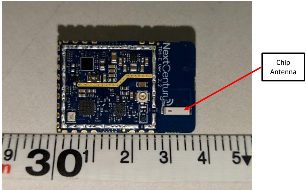
Photograph 1 – Front View of the EUT, Shield Removed
