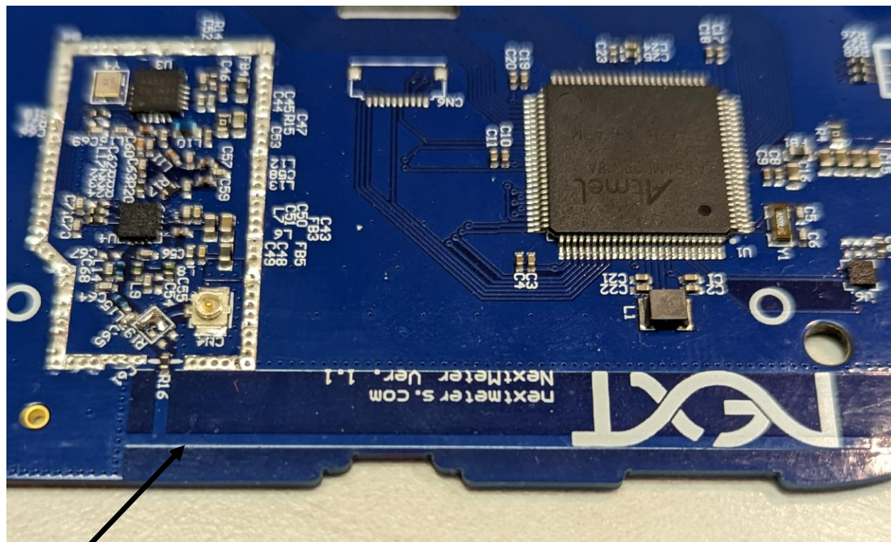
Photograph 3 – View of Circuitry Under the RF Shield
