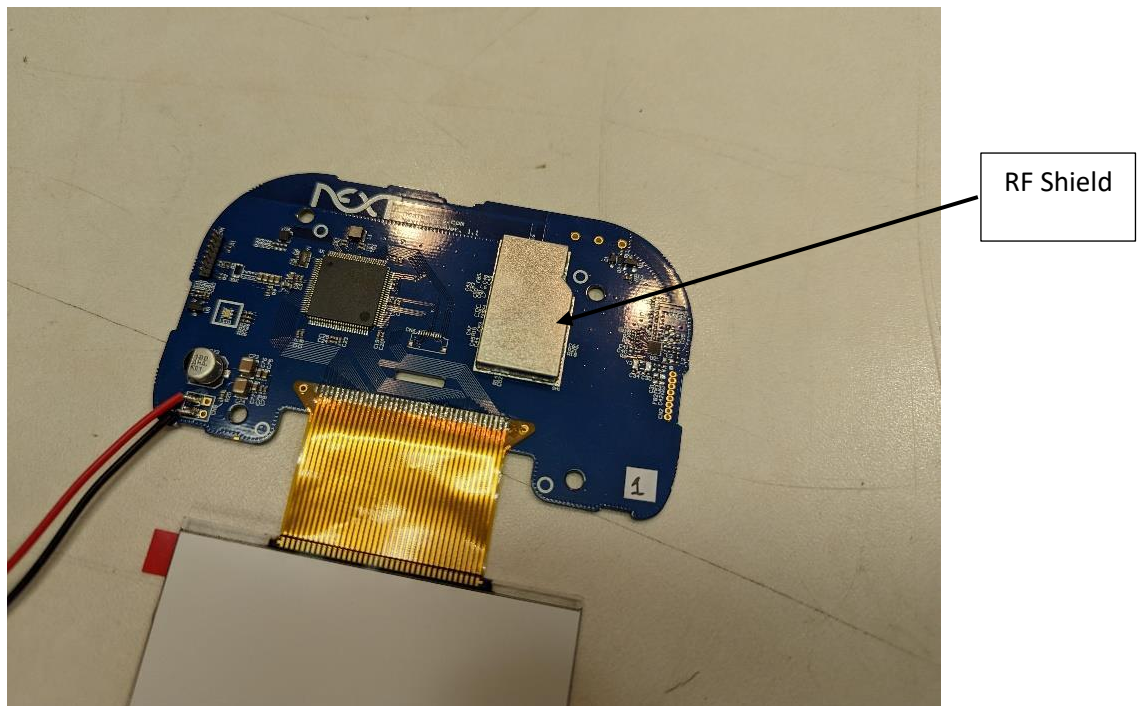
Photograph 1 – Front View of the Device with RF Shield
