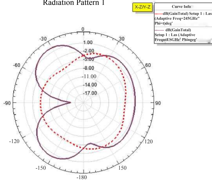
Radiation Pattern 1
