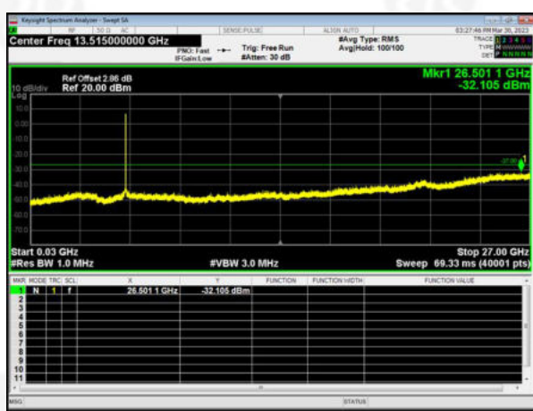
802.11n20 on channel 36
