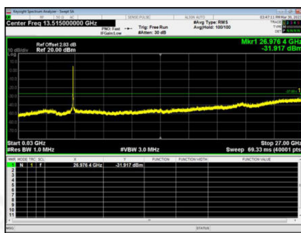
802.11n40 on channel 46
