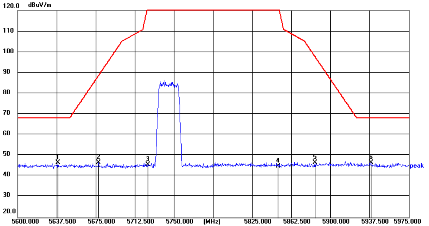
802.11ax20_Low channel_Horizontal
