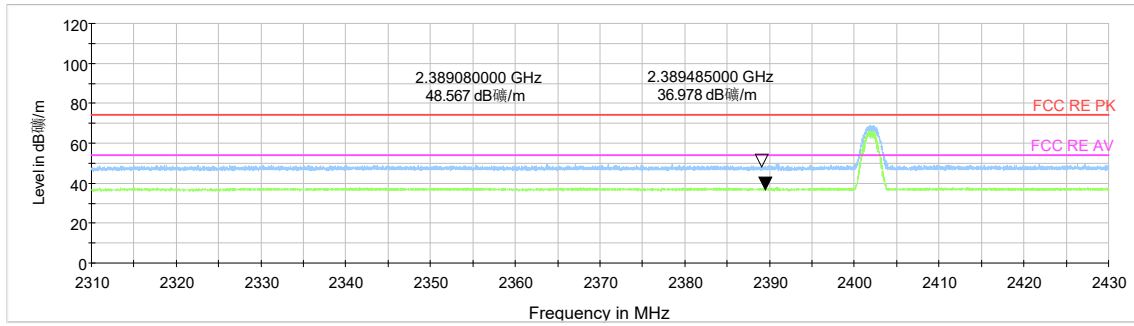
Bluetooth LE Channel 0 Peak+ Average
