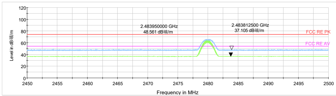
Bluetooth LE Channel 39 Peak+Average
